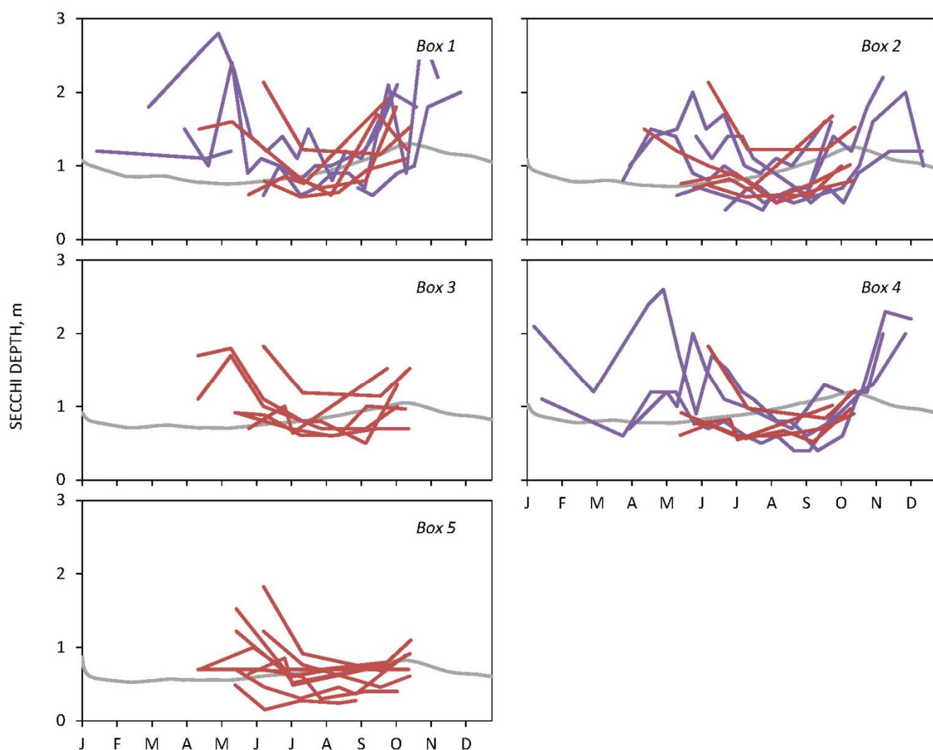
Fig. A11. Simulated secchi depth (grey) in each spatial element with data from multiple years from MDDNR (purple) and UMCES (red).
