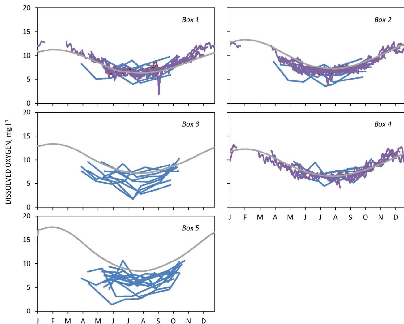
Fig. A10. Simulated DO (grey) in each spatial element with data from multiple years from MDDNR (purple), UMCES (red), and the Riverkeeper (blue).
