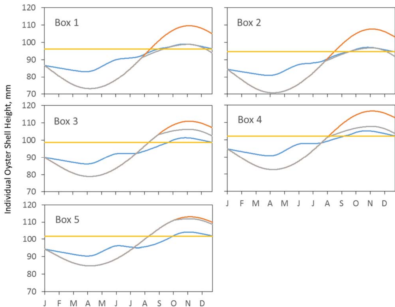
Fig. 11. Simulated annual growth trajectories of oyster shell height in each box (blue), with von Bertalanffy growth trajectories from Liddel (2008) without (red) and with (grey) the effects of parasitism, and projected final shell height based on data from the Choptank River (yellow, Kellogg and Paynter, unpublished data).
