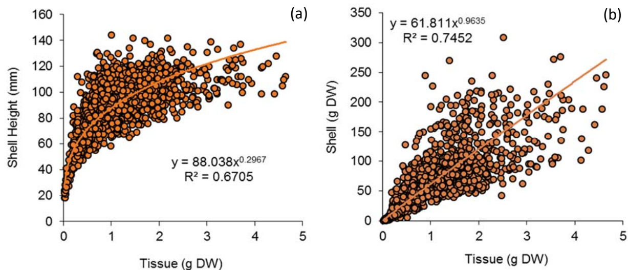
Fig. 4. Relationship between individual oyster tissue weight and individual shell (a) height and (b) weight fit to data from Harris Creek.
