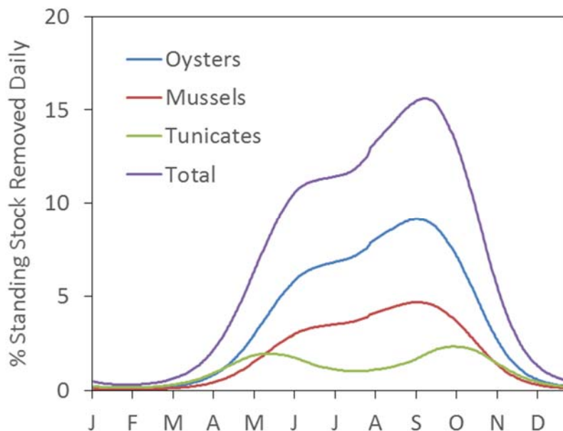
Fig. 20. Modeled daily removal of TSS expressed as a percent of the standing stock.
