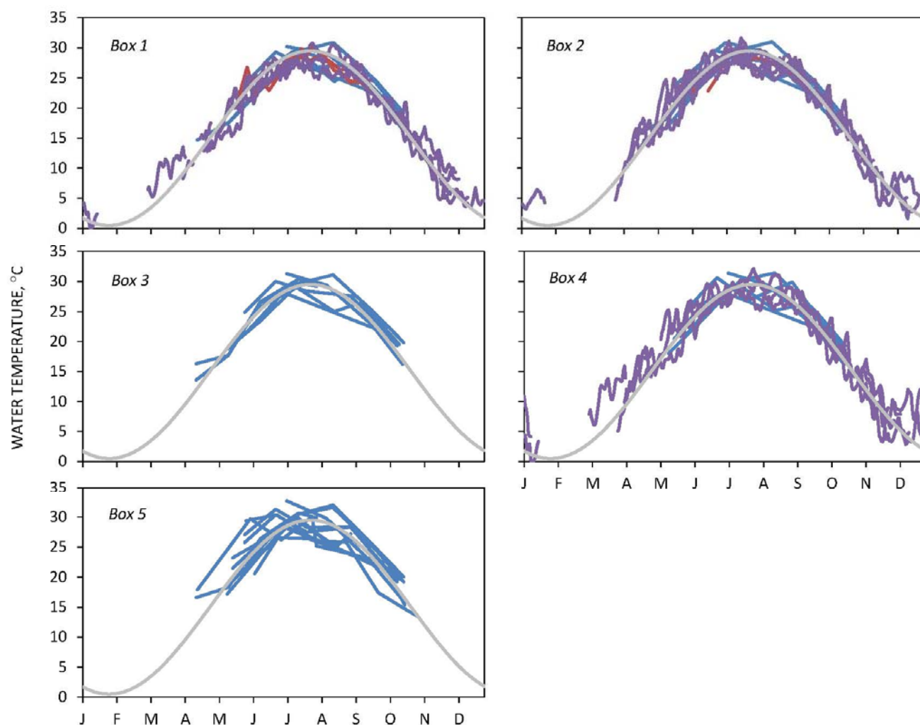
Fig. A5. Model forcing functions for water temperature (grey lines), fit to data from multiple years from MDDNR (purple), UMCES (red), and the Riverkeeper (blue).
