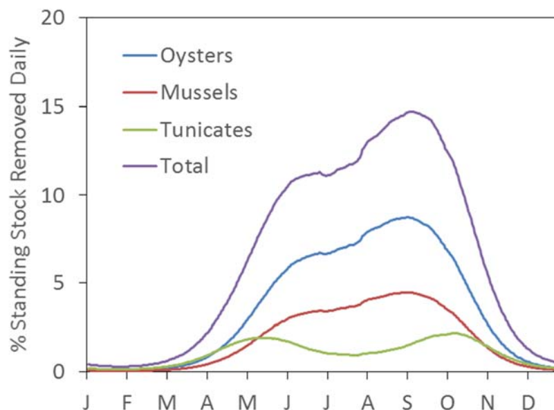
Fig. 19. Modeled daily removal of chl-a expressed as a percent of the standing stock.
