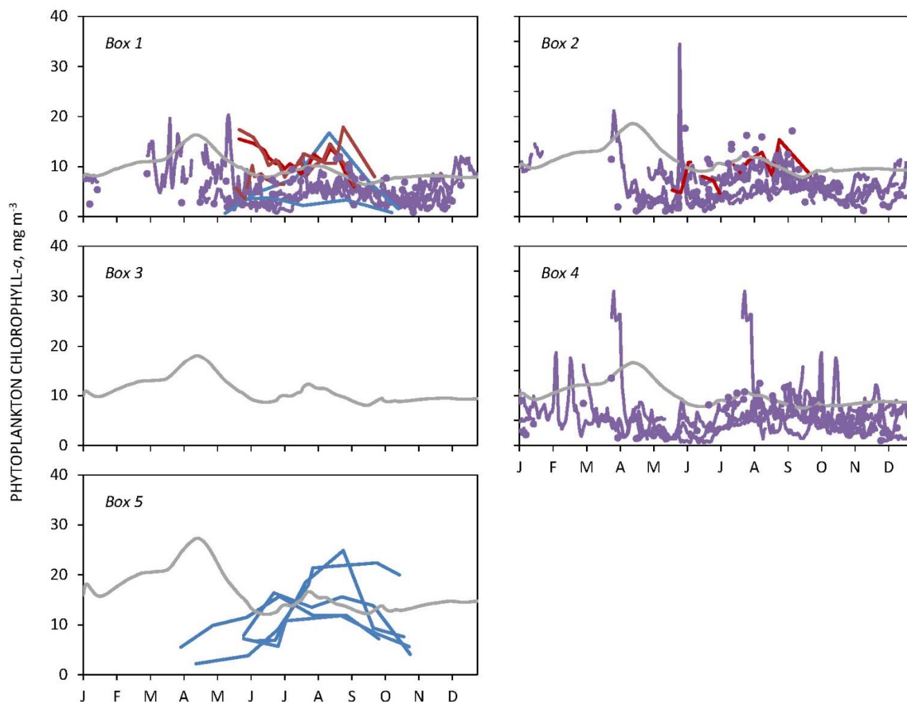
Fig. A8. Simulated chlorophyll-a (grey) in each spatial element with data from multiple years from MDDNR (purple), UMCES (red), and the Riverkeeper (blue). MDDNR high frequency sonde data are shown with continuous lines, while data from calibration cruises are shown with points.
