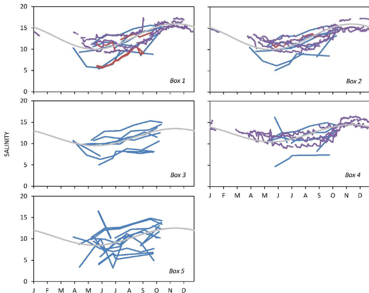
Fig. A6. Model forcing functions for salinity (grey lines), fit to data from multiple years from MDDNR (purple), UMCES (red), and the Riverkeeper (blue).
