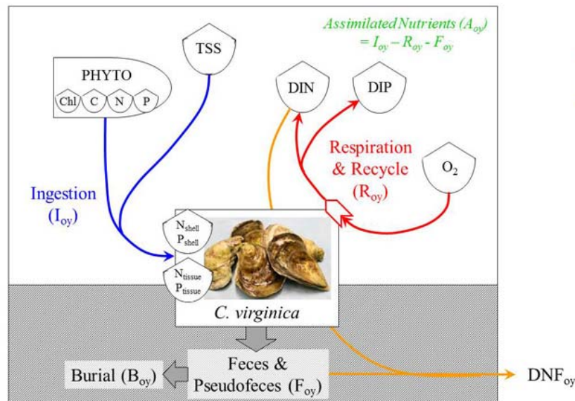
Fig. 3. Oyster submodel with linkages to the base ecosystem model in Fig. 2. Photo: New York State Department of Environmental Conservation.
