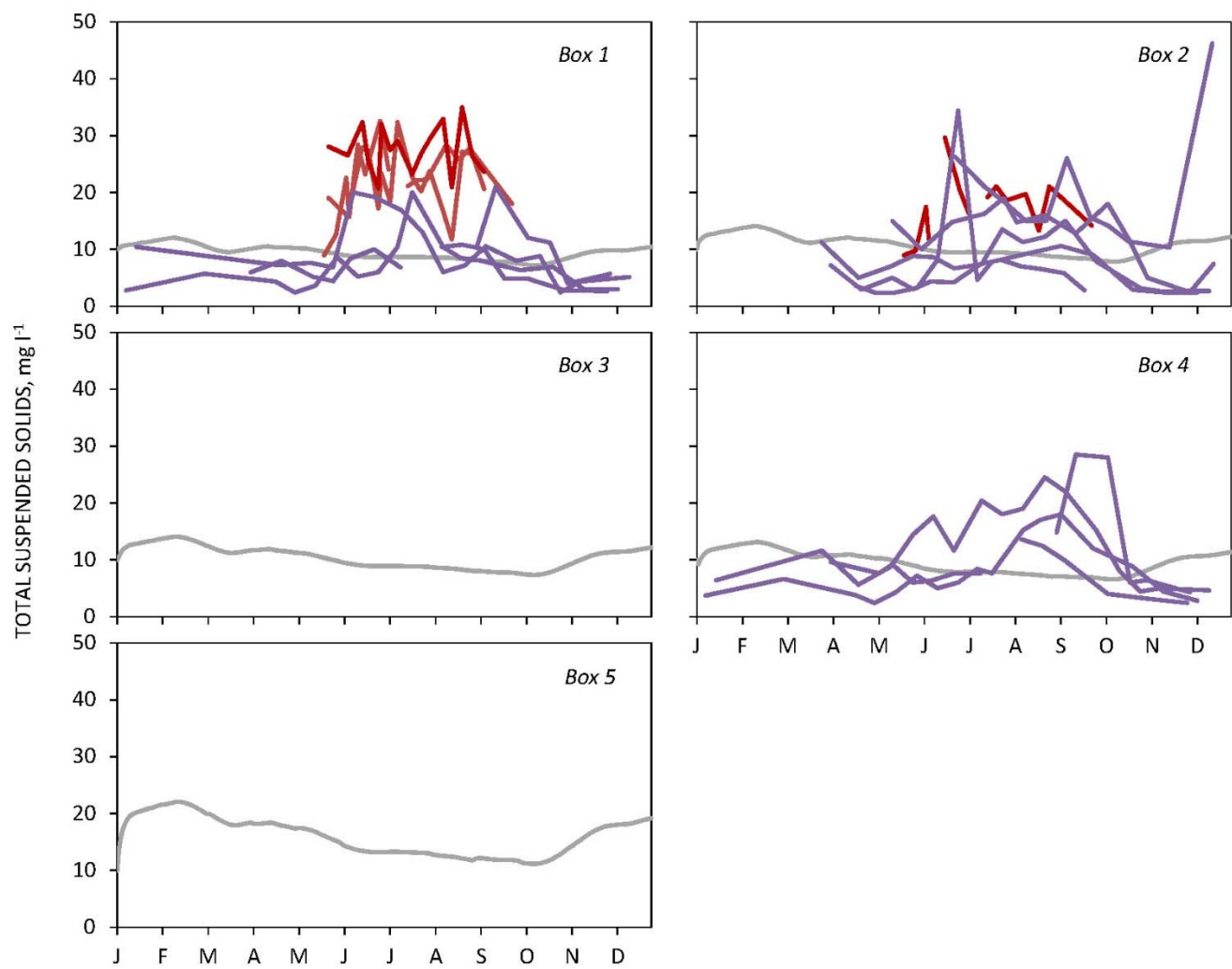
Fig. A9. Simulated TSS (grey) in each spatial element with data from multiple years from MDDNR (purple) and UMCES (red).
