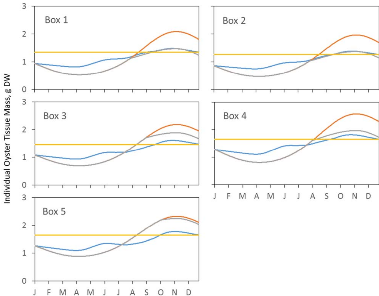
Fig. 10. Simulated annual growth trajectories of oyster tissue DW in each box (blue), with von Bertalanffy growth trajectories from Liddel (2008) without (red) and with (grey) the effects of parasitism, and projected final DW based on data from the Choptank River (yellow, Kellogg and Paynter, unpublished data).
