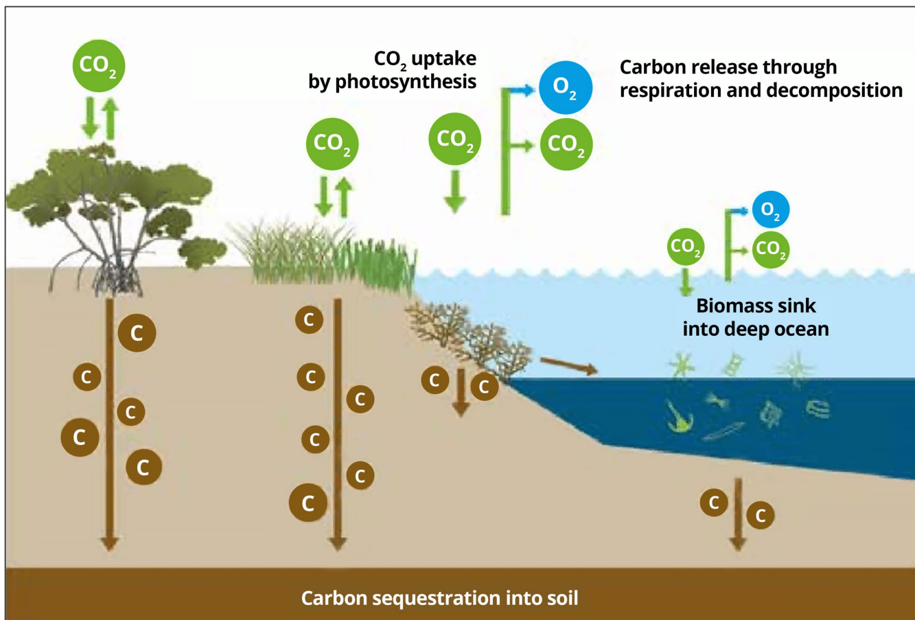
Figure 1. Graphic illustration of blue carbon ecosystems' carbon uptake via photosynthesis and subsequent long-term sequestration into biomass and soil, or release into the atmosphere via respiration.
