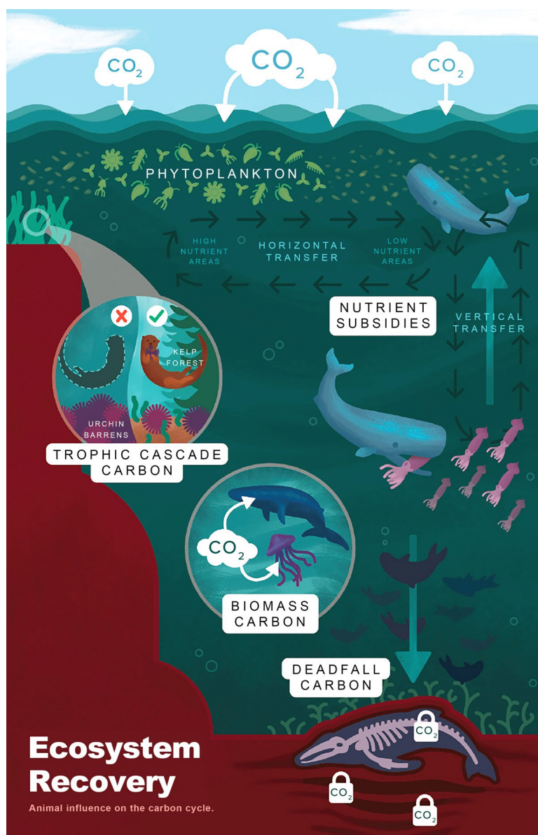
Figure 4. Animal influence on the marine carbon cycle.
