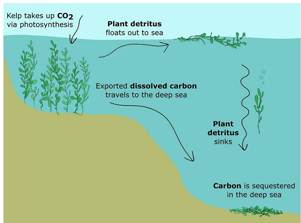
Figure 3. Seaweed carbon production and export in the nearshore ocean.
