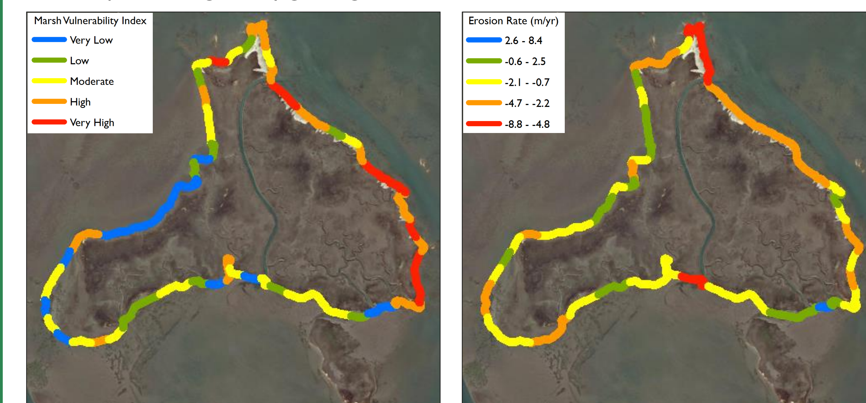
Figure 7. Comparison between MVI output (left) and shoreline erosion rates (right) (2009 - 2014) at Man and Boy Marsh. Areas of high (low) risk generally correspond with areas of higher (lower) shoreline erosion.
