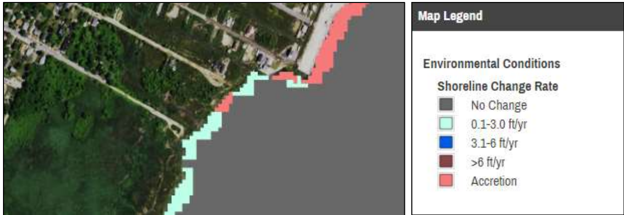
Figure 11. Average erosion rate of project sites (from 1977-2012).
