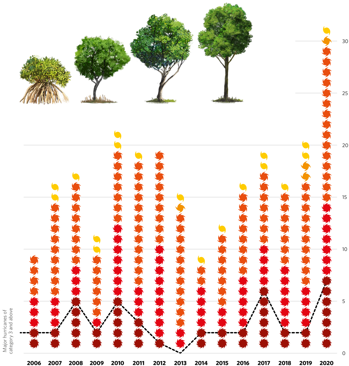
Figure 5: Number and intensity of tropical storm events per season in the Gulf of Mexico and Caribbean.
