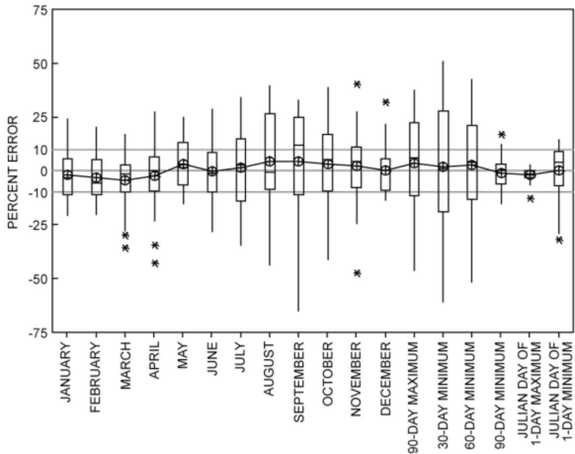
Figure 8. Percent error between observed and estimated monthly mean flows and other ecologically-relevant streamflow statistics at the 31 validation streamgauges.
