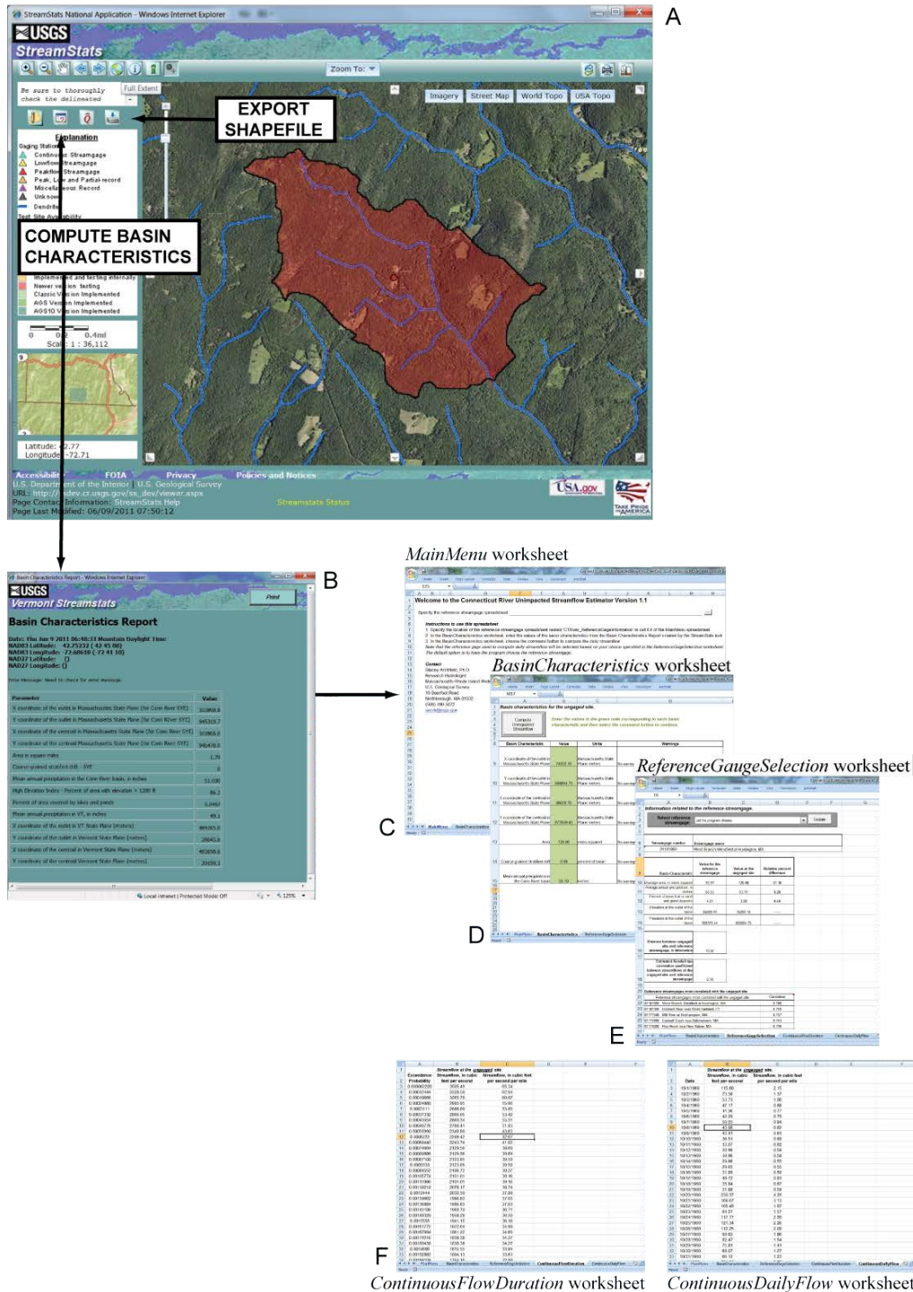
Figure 5. Screen captures showing the decision-support tool used to estimate daily, unregulated time series in the Connecticut River Basin. The program delineates a catchment for the ungauged location selected by the user (A) and summarizes the catchment characteristics (B). The user then inputs these characteristics into a spreadsheet program (C-E) that generates the daily, period of record flow-duration curve (F) and the daily streamflow time series (G).
