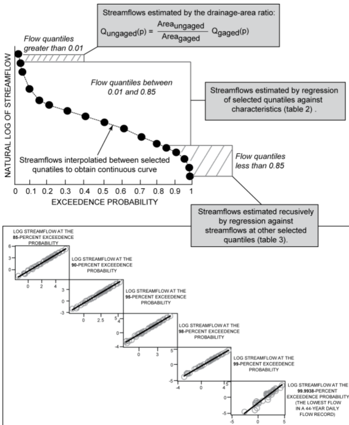
Figure 4. Diagram showing the methods used to estimate a continuous, daily flow duration at an ungaged location.
