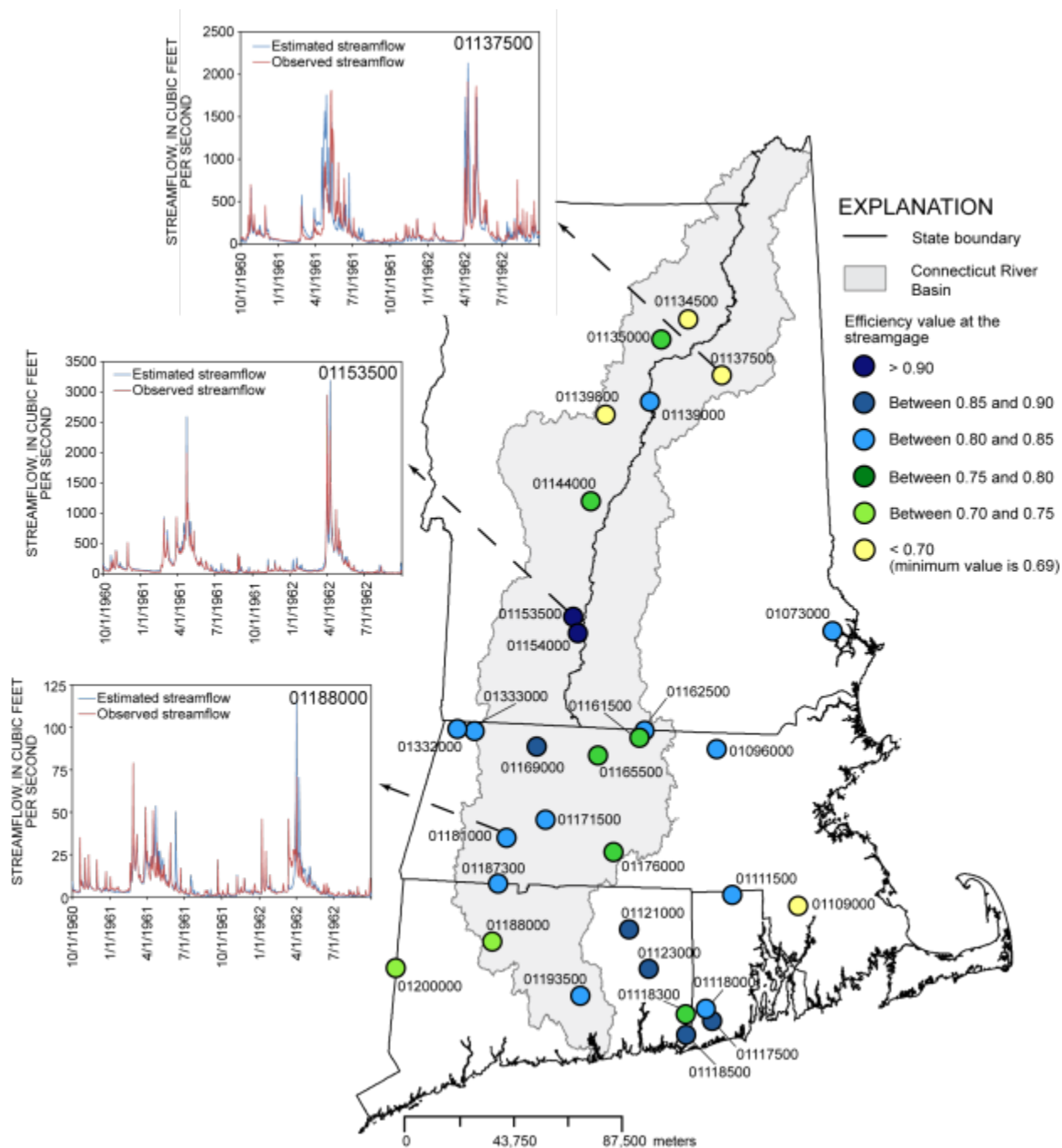
Figure 7. Spatial distribution of efficiency values resulting from log-transformed observed and estimated daily streamflow at 31 validation streamgages and selected hydrographs of observed and estimated streamflow for the period from October 1, 1960 through September 30, 1962.
