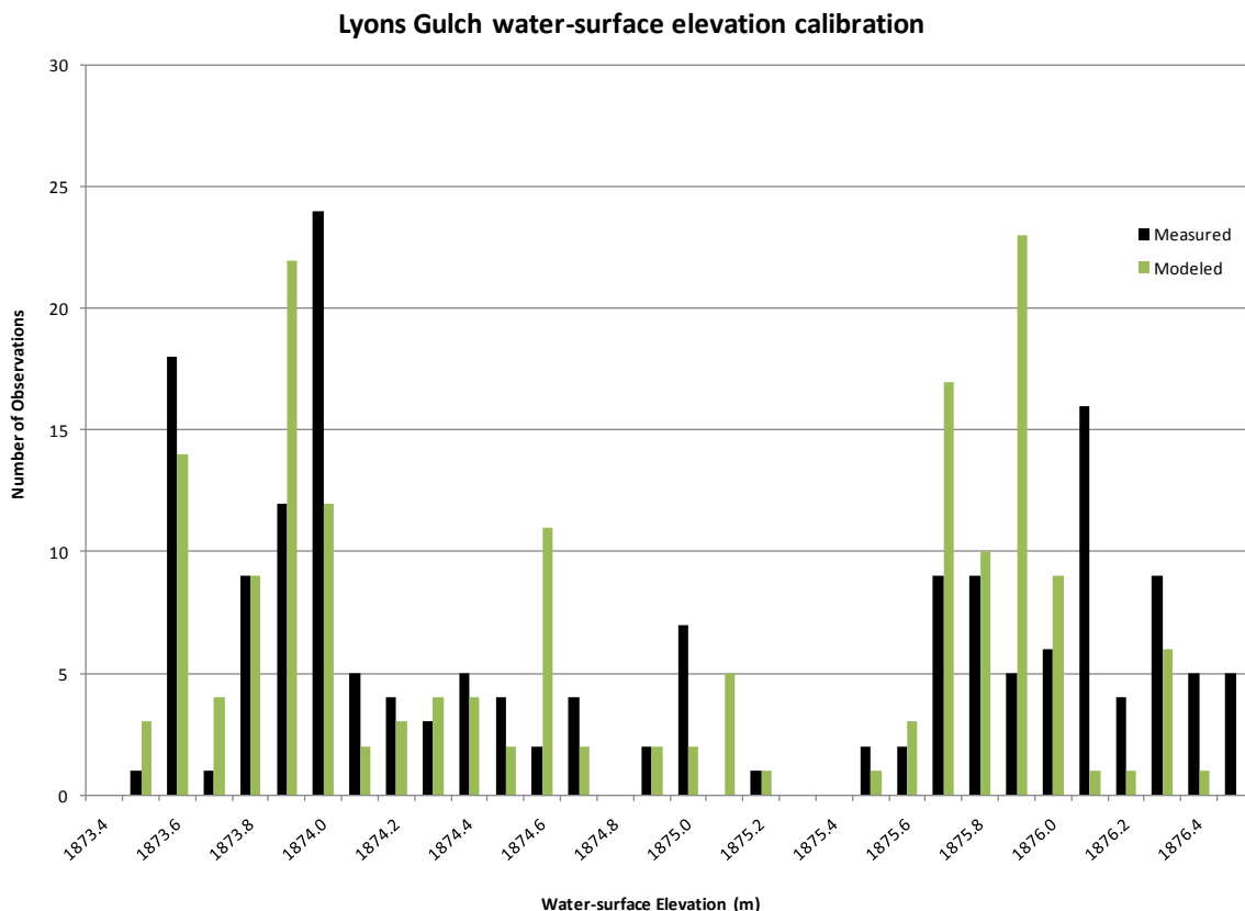
Figure 23. Example of measured versus modeled water-surface elevations for low flow at Lyons Gulch.
