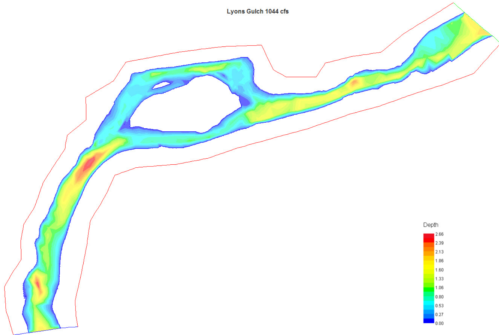
Figure 50. Lyons Gulch simulated water depth (m) at 1044 cfs (low flow). Flow moves from right to left.
