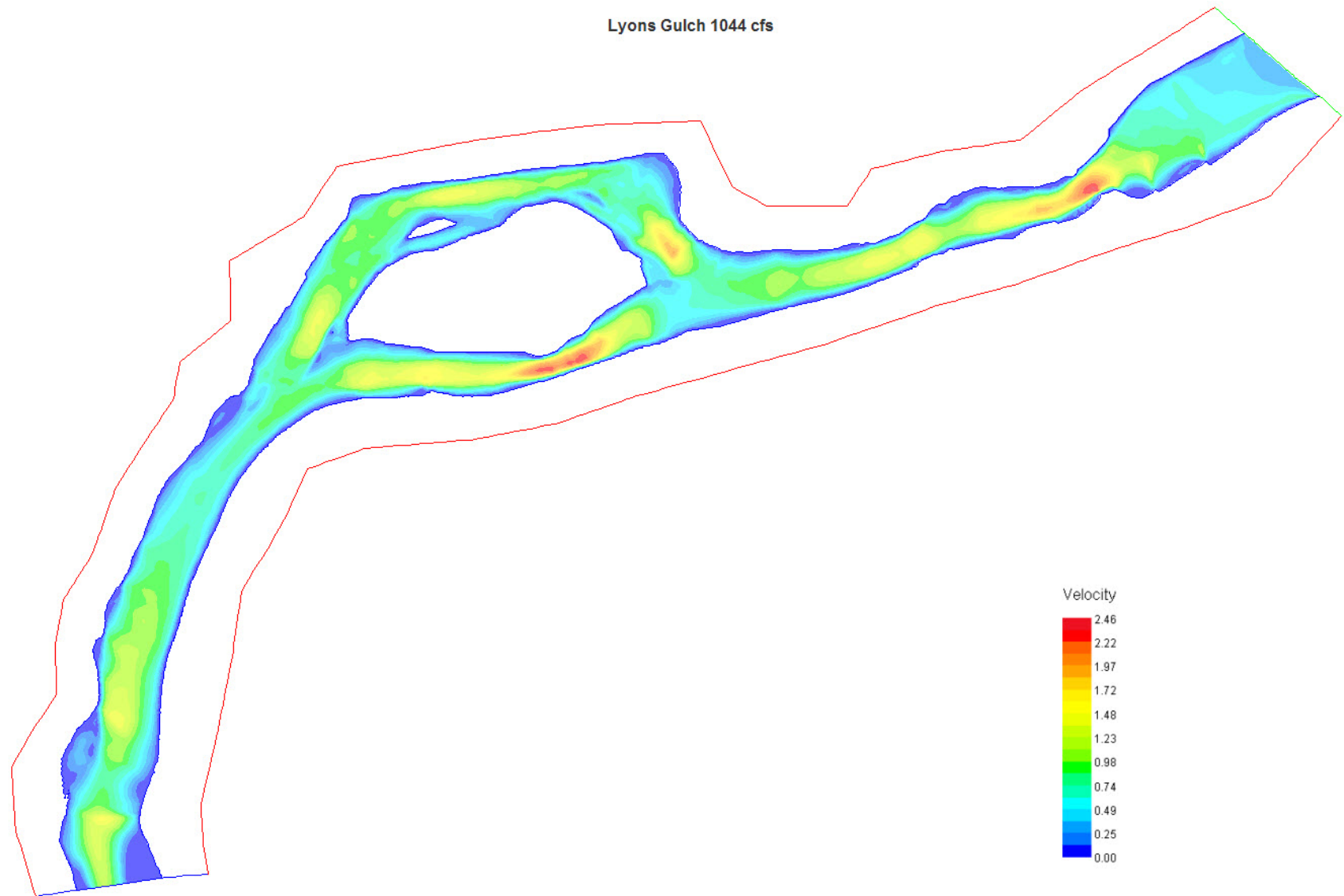
Figure 48. Lyons Gulch simulated water velocity (m/s) at 1044 cfs (low flow). Flow moves from right to left.
