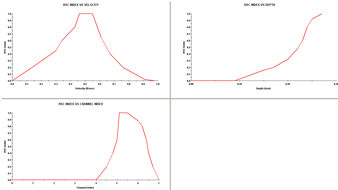
Figure 27. Mountain whitefish spawning HSI
