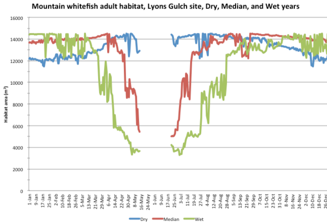
Figure 81. Adult mountain whitefish habitat at Lyons Gulch in dry, median, and wet years.
