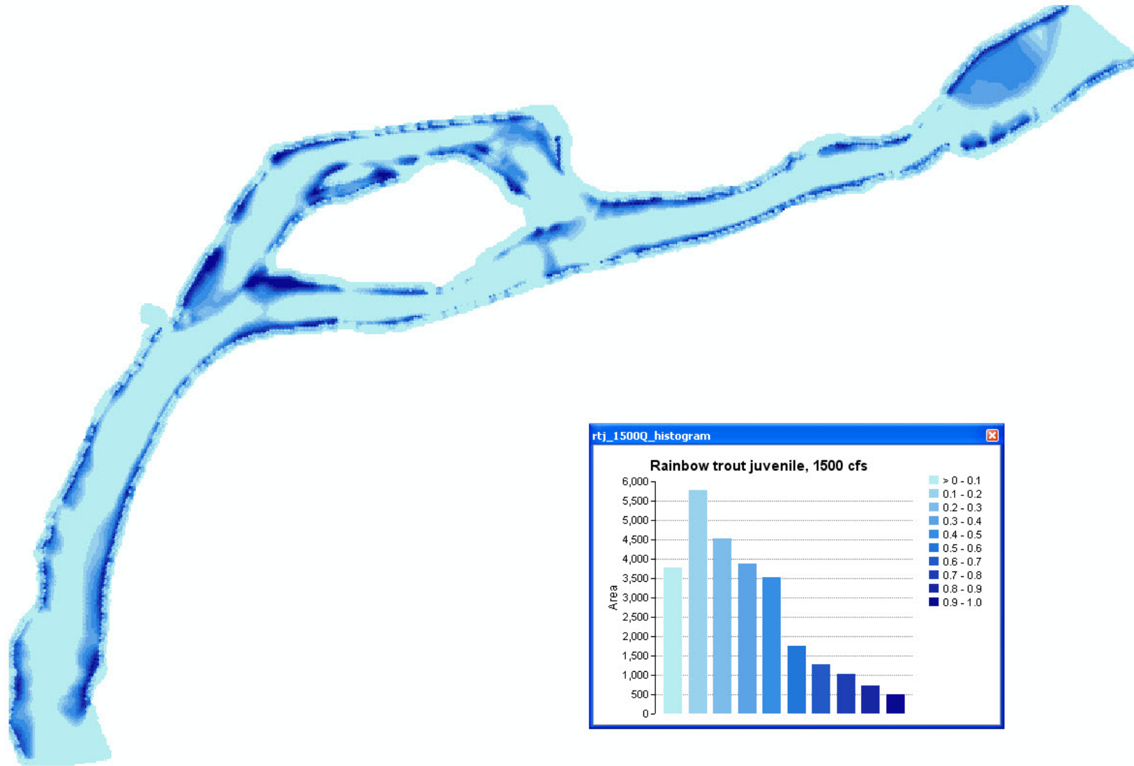
Figure A-73. Juvenile rainbow trout habitat map, Lyons Gulch site, 1500 cfs.
