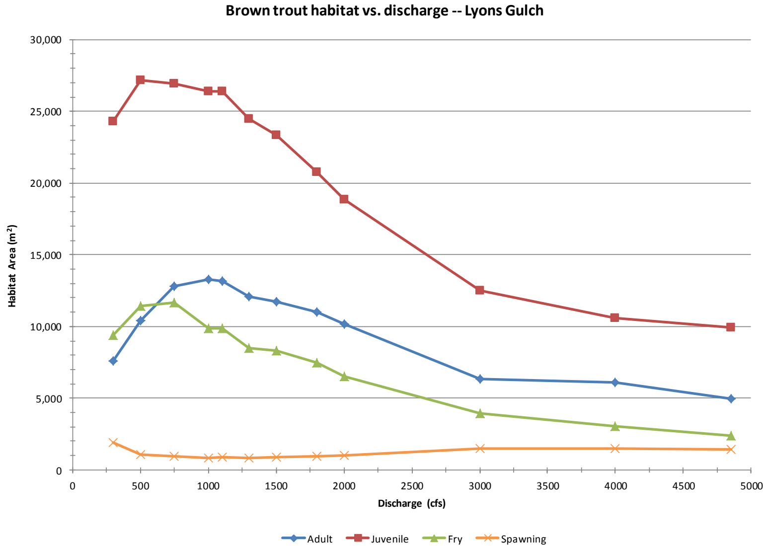
Figure 75. Brown trout habitat versus discharge, Lyons Gulch site.
