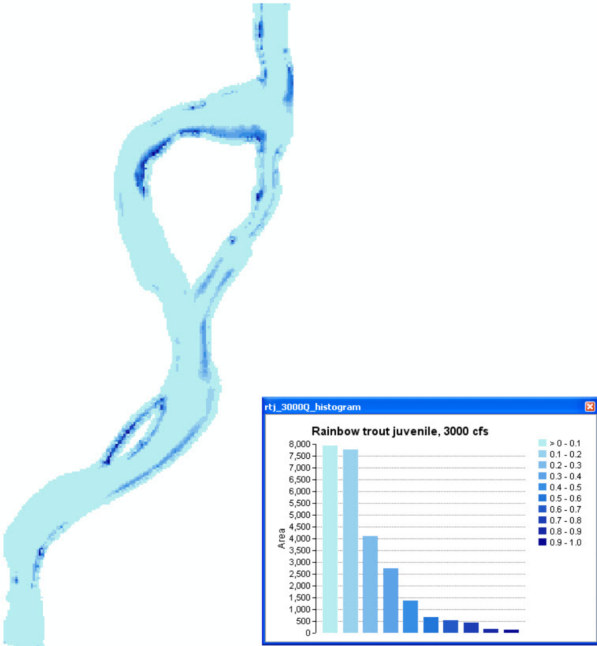
Figure A-41. Juvenile rainbow trout habitat map, Rancho del Rio site, 3000 cfs.
