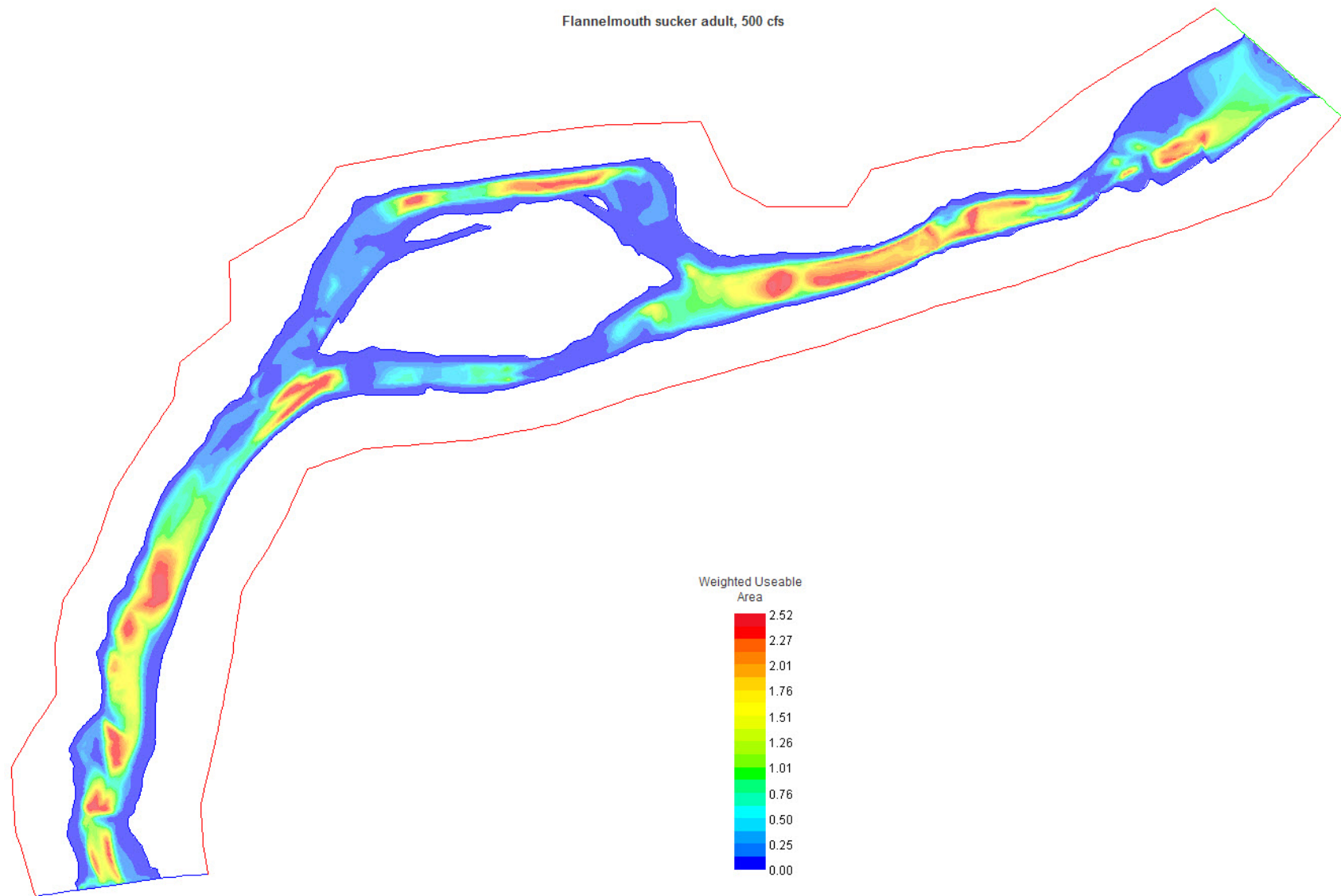
Figure A-93. Adult flannelmouth sucker habitat map, Lyons Gulch site, 500 cfs.
