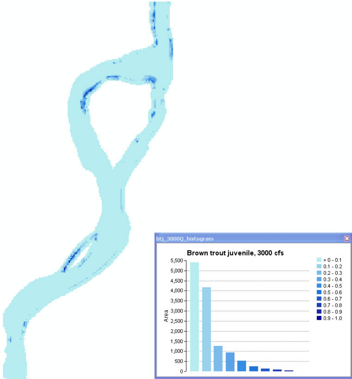
Figure A-35. Juvenile brown trout habitat map, Rancho del Rio site, 3000 cfs.
