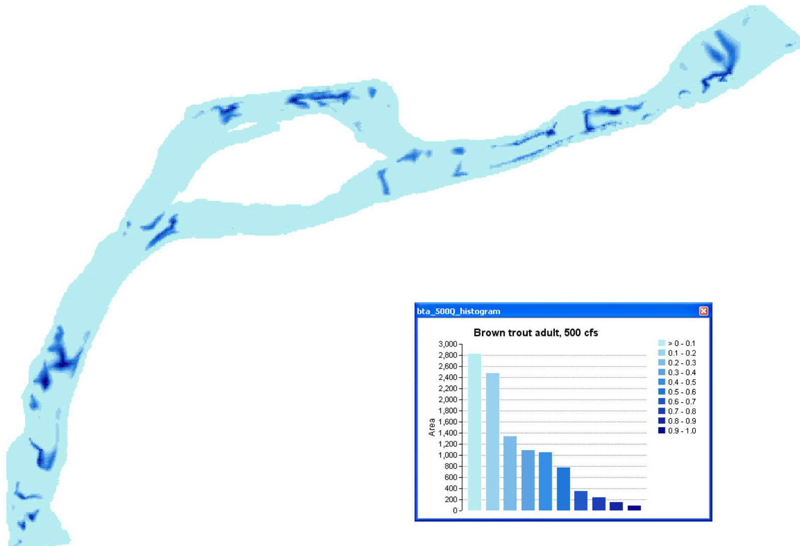
Figure A-63. Adult brown trout habitat map, Lyons Gulch site, 500 cfs.
