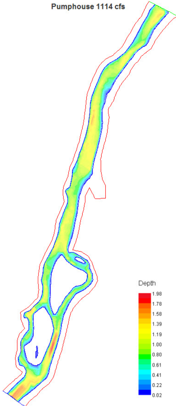
Figure E-1. Example of depth simulation in River2D. Depth is in meters, river flows from top of page to bottom, red line is model boundary.
