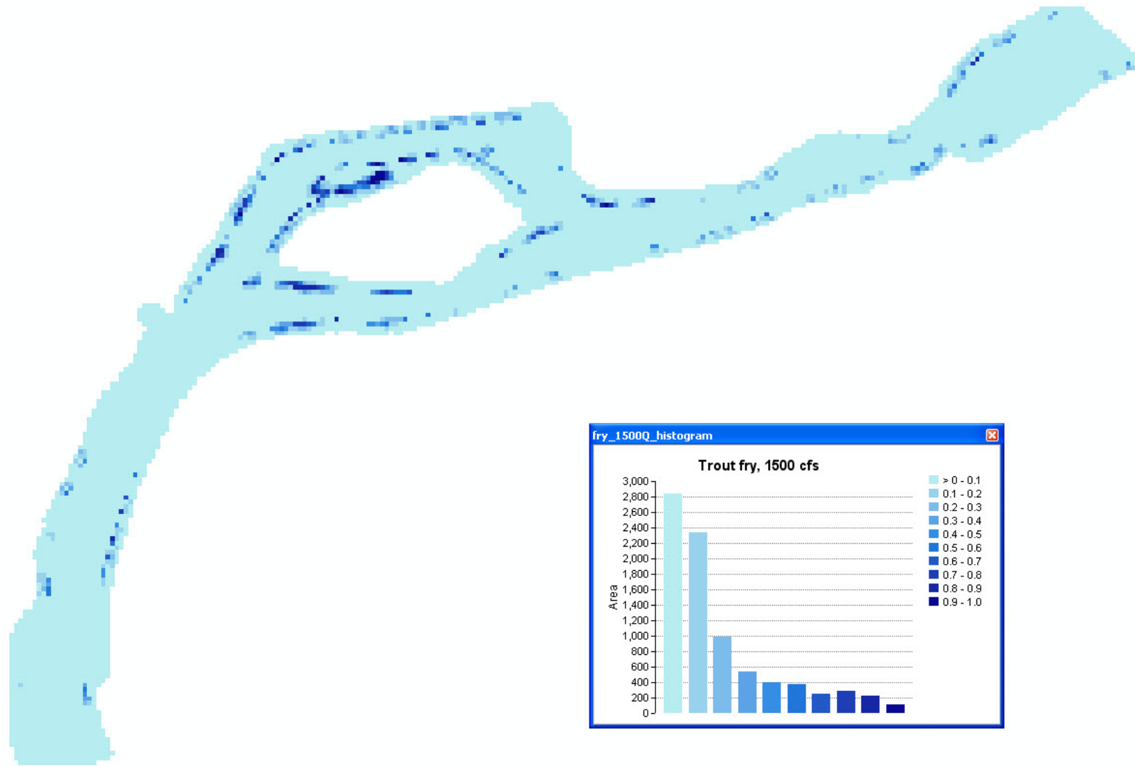
Figure A-76. Trout fry habitat map, Lyons Gulch site, 1500 cfs.
