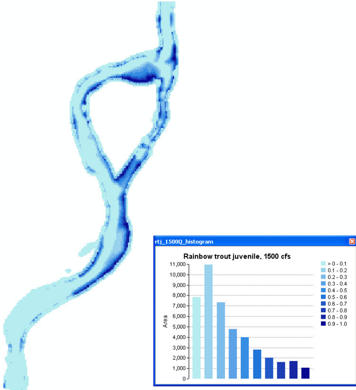
Figure A-40. Juvenile rainbow trout habitat map, Rancho del Rio site, 1500 cfs.
