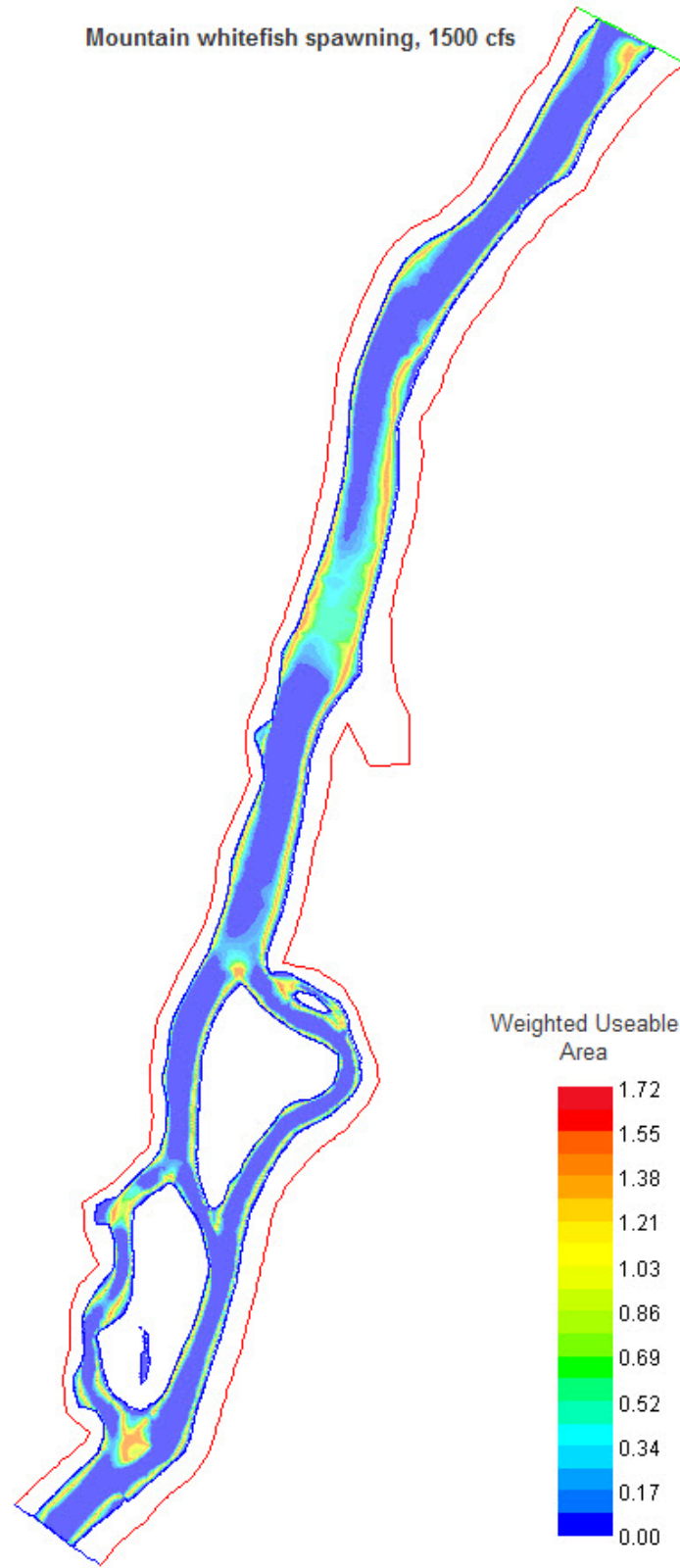
Figure A-28. Mountain whitefish spawning habitat map, Pumphouse site, 1500 cfs.
