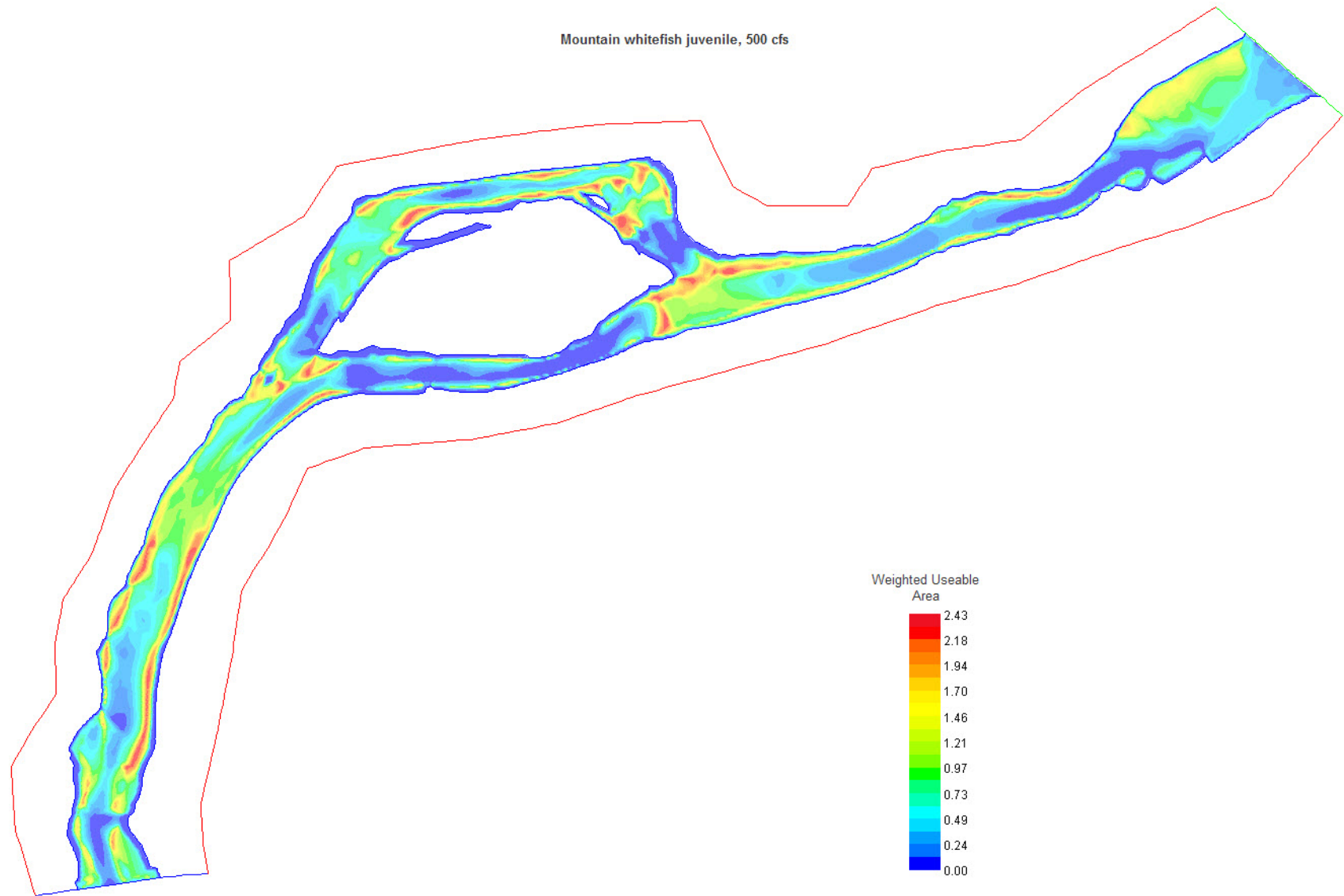
Figure A-84. Juvenile mountain whitefish habitat map, Lyons Gulch site, 500 cfs.
