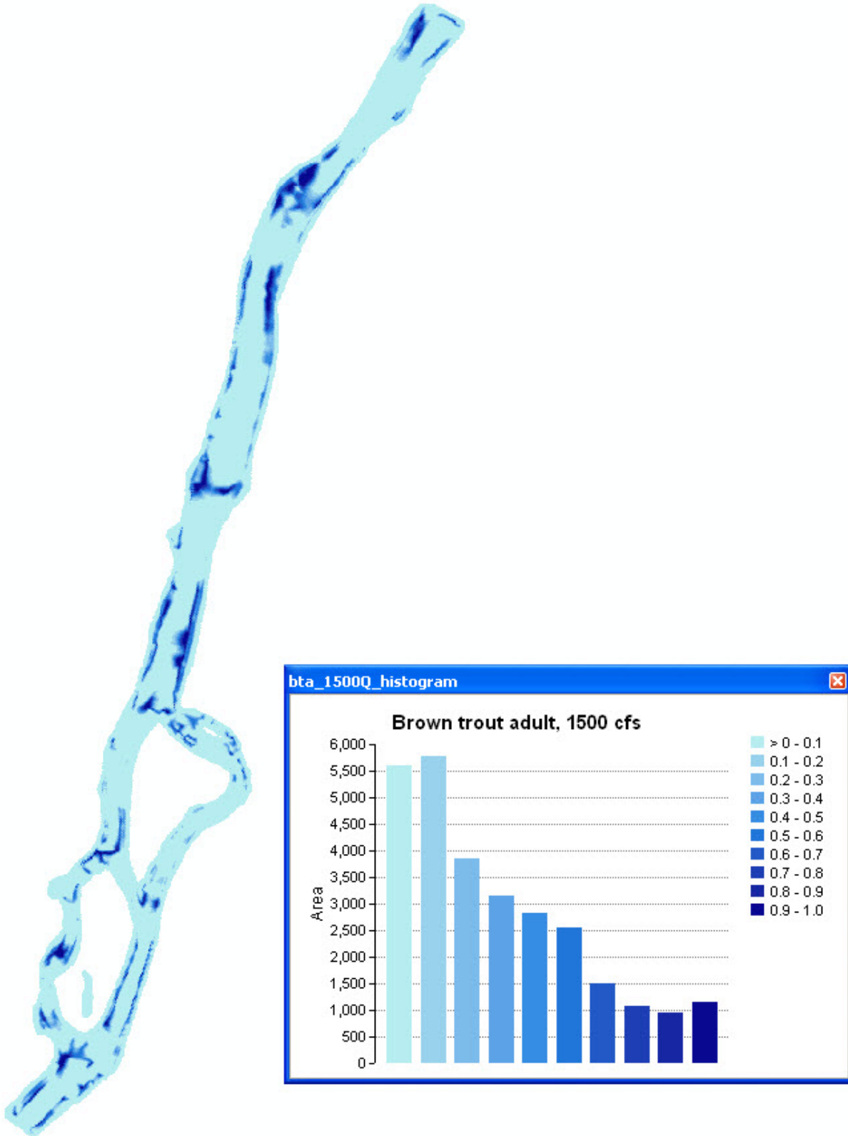
Figure A-2. Adult brown trout habitat map, Pumhouse site, 1500 cfs.
