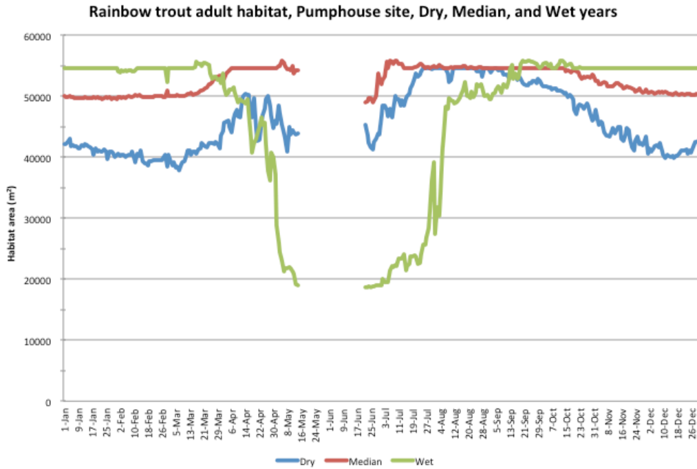
Figure 62. Adult rainbow trout habitat at the Pumphouse site in dry, median, and wet years.
