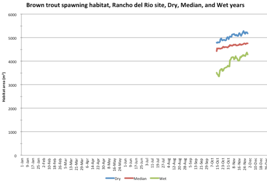
Figure B-16. Brown trout spawning habitat time series, dry, median, and wet years, Rancho del Rio site.
