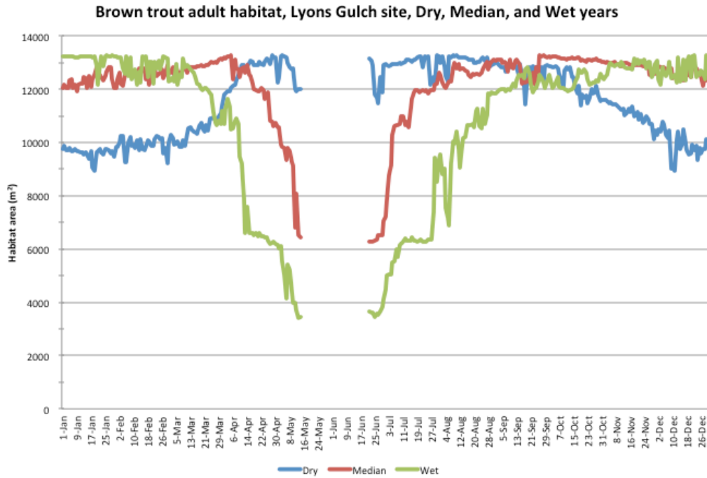
Figure B-26. Adult brown trout habitat time series, dry, median, and wet years, Lyons Gulch site.
