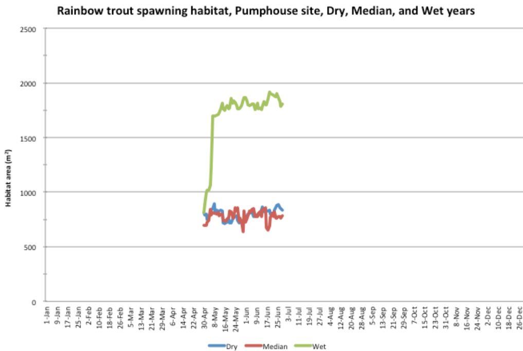
Figure B-8. Rainbow trout spawning habitat time series, dry, median, and wet years, Pumphouse site.
