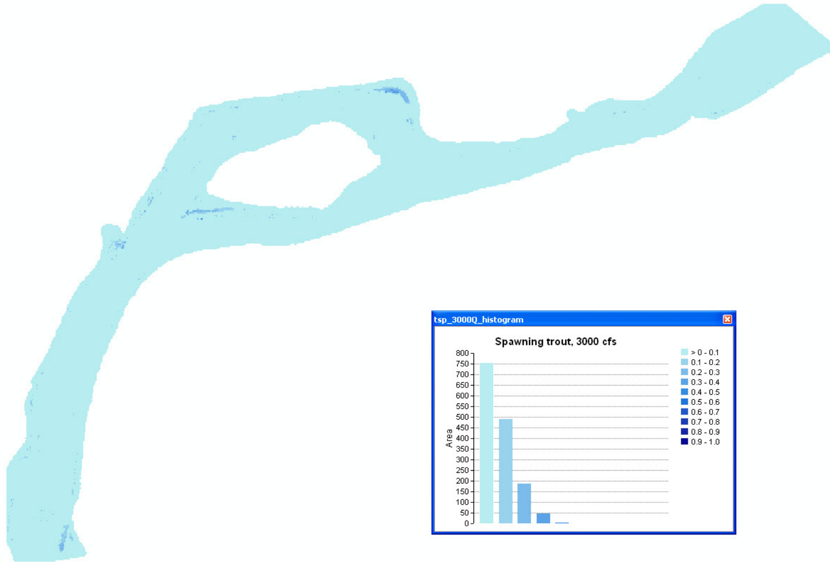
Figure A-80. Trout spawning habitat map, Lyons Gulch site, 3000 cfs.
