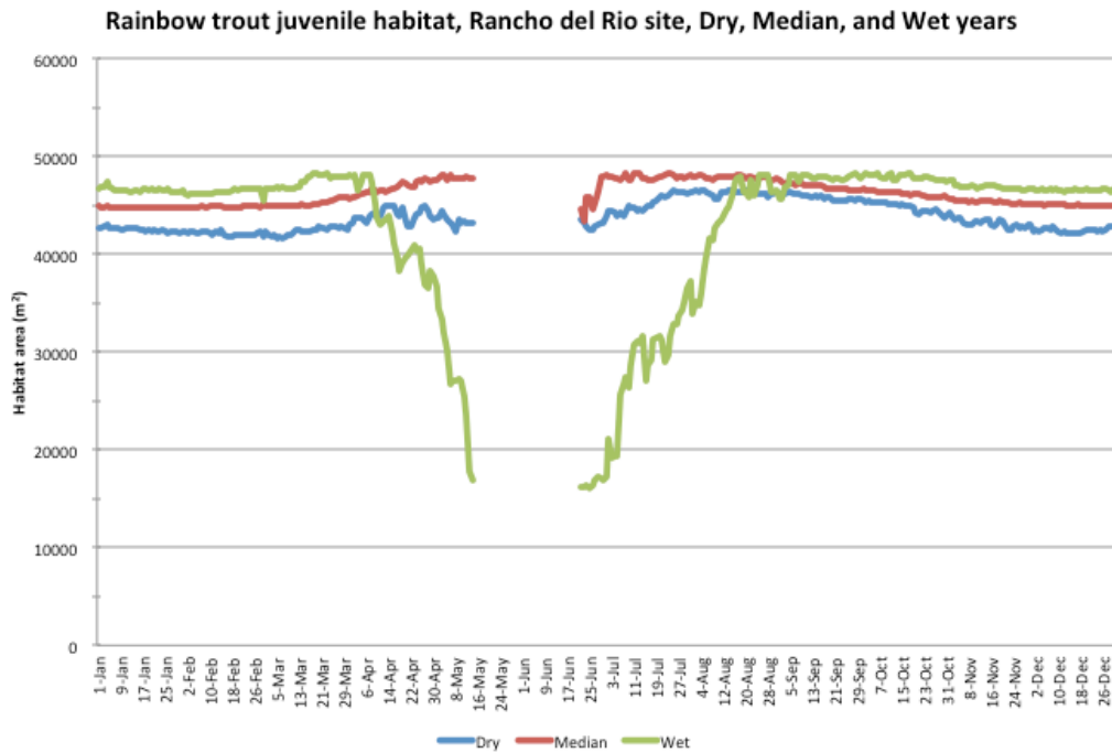
Figure B-18. Juvenile rainbow trout habitat time series, dry, median, and wet years, Rancho del Rio site.
