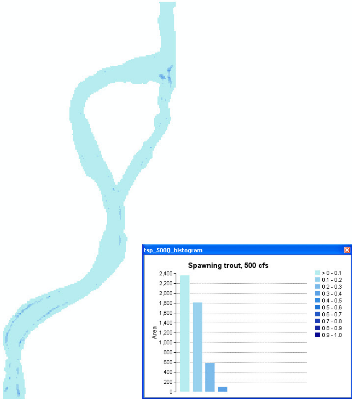
Figure A-45. Trout spawning habitat map, Rancho del Rio site, 500 cfs.
