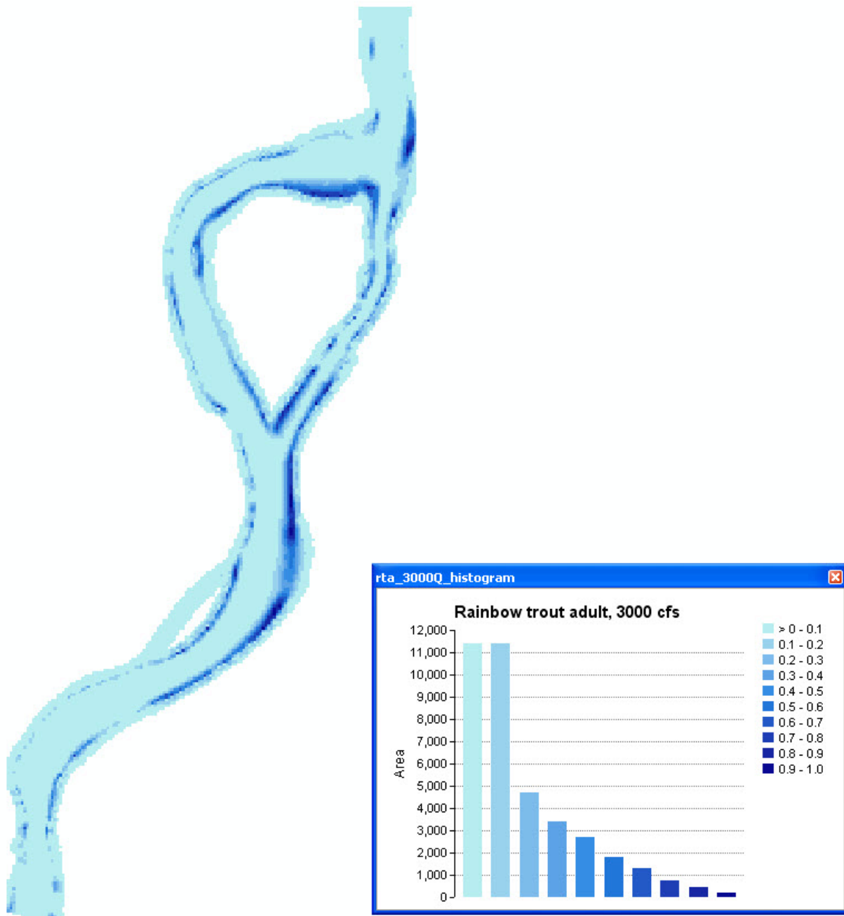
Figure 68. Adult rainbow trout habitat map at 3000 cfs at Rancho del Rio.
