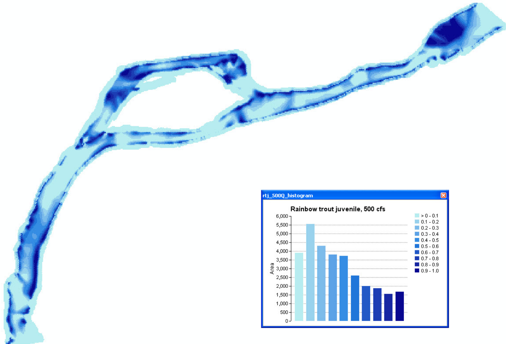
Figure A-72. Juvenile rainbow trout habitat map, Lyons Gulch site, 500 cfs.
