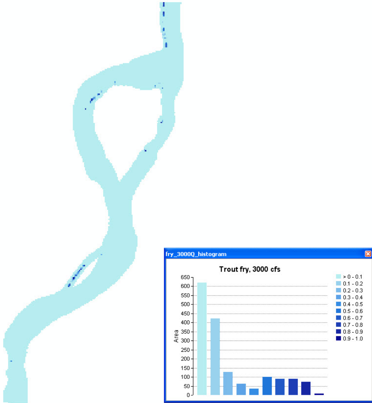
Figure A-44. Trout fry habitat map, Rancho del Rio site, 3000 cfs.
