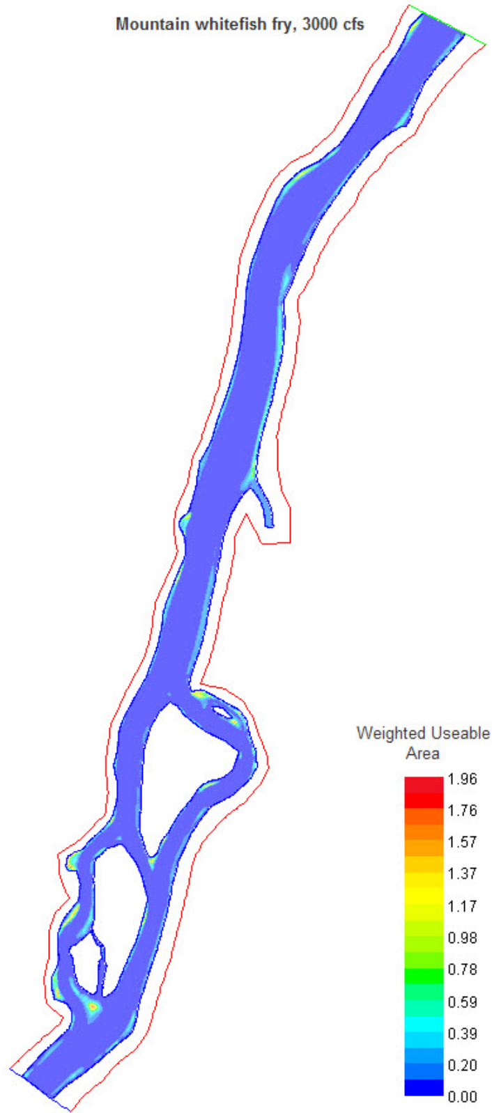
Figure A-26. Mountain whitefish fry habitat map, Pumphouse site, 3000 cfs.
