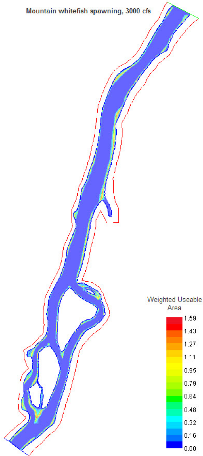
Figure A-29. Mountain whitefish spawning habitat map, Pumphouse site, 3000 cfs
