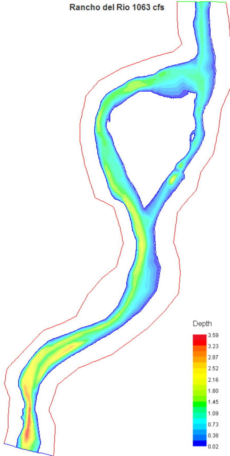
Figure 43. Rancho del Rio simulated water depth (m) at 1063 cfs (low flow). Flow moves from top to bottom.
