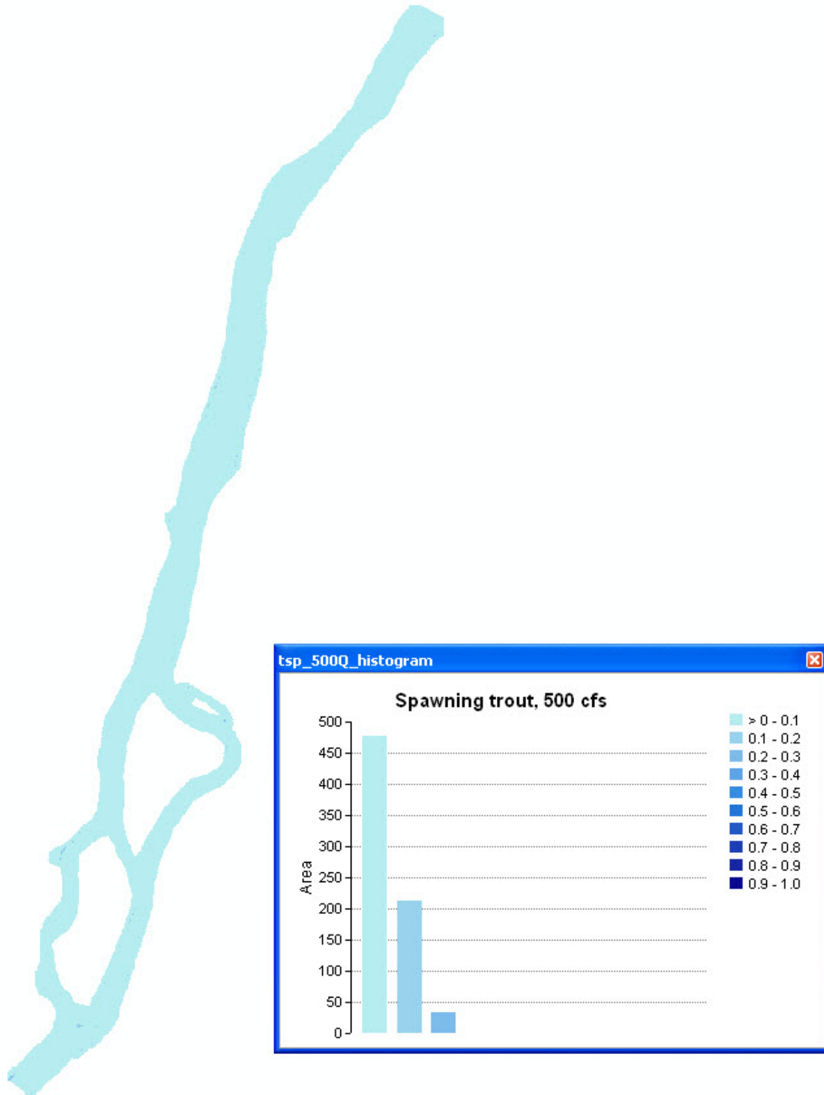
Figure A-16. Trout spawning habitat map, Pumphouse site, 500 cfs.
