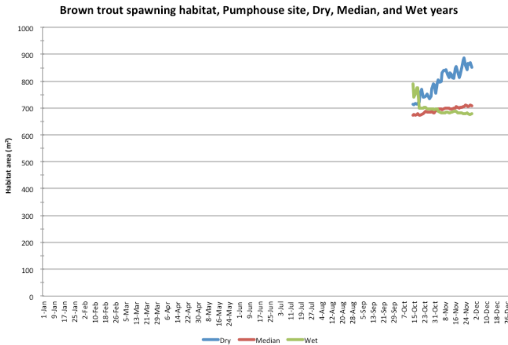
Figure B-4. Brown trout spawning habitat time series, dry, median, and wet years, Pumphouse site.
