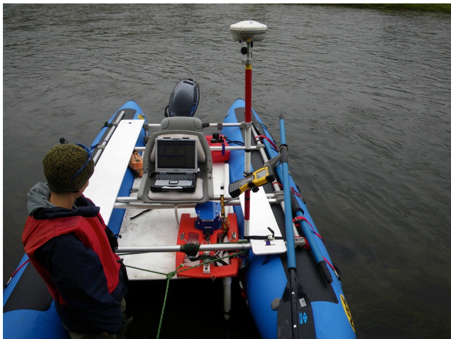
Figure 13. Setup of the ADCP, GPS rover unit, and laptop computer on a raft so that bed elevations and velocities can be measured.
