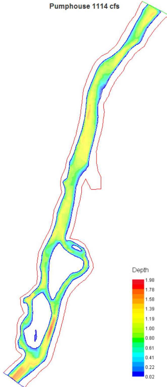
Figure 31. Pumphouse simulated water depth (m) at 1114 cfs (low flow). Flow moves from top to bottom.
