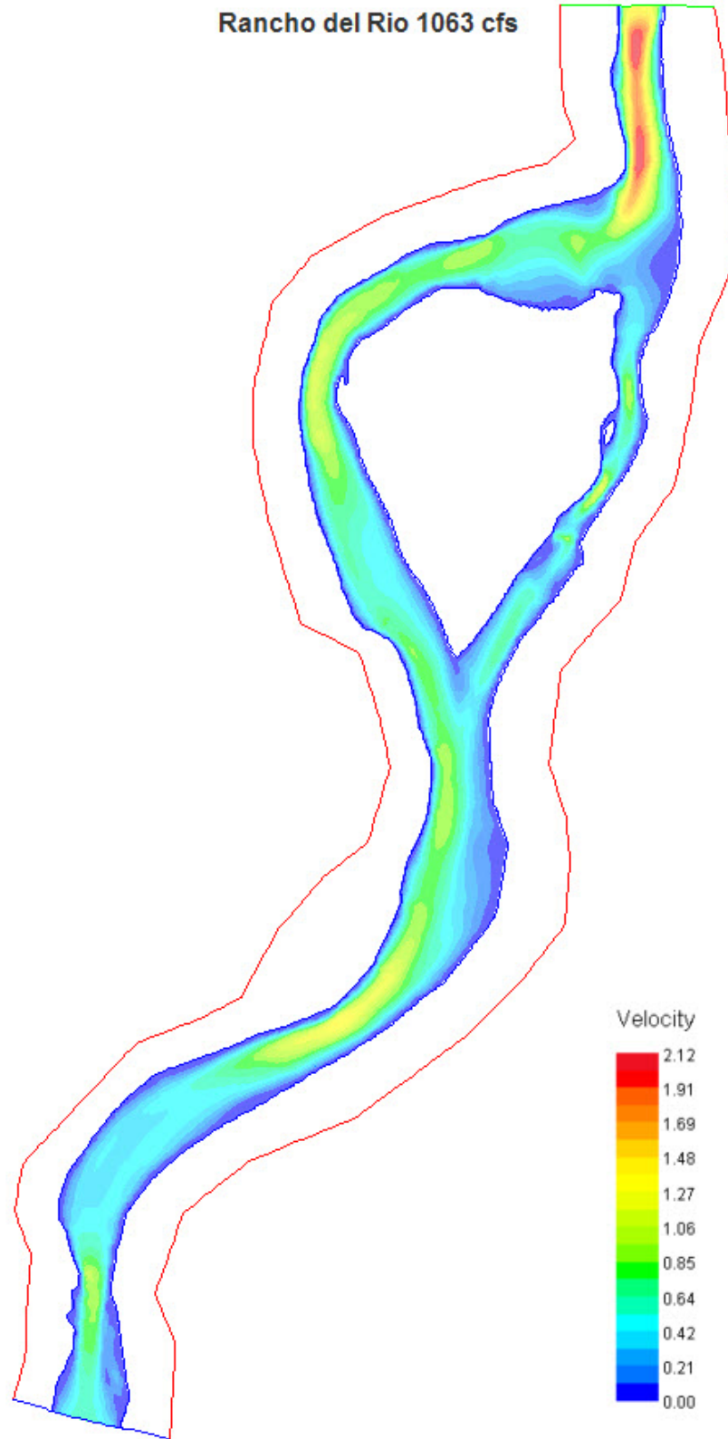
Figure 41. Rancho del Rio simulated water velocity (m/s) at 1063 cfs (low flow). Flow moves from top to bottom.
