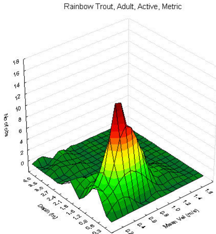
Figure 16. Example of a three-dimensional surface used to generate a habitat suitability equation for adult rainbow trout.
