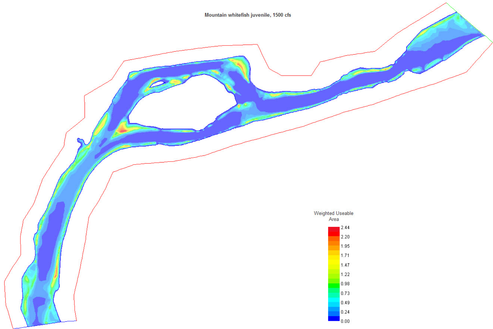
Figure A-85. Juvenile mountain whitefish habitat map, Lyons Gulch site, 1500 cfs.
