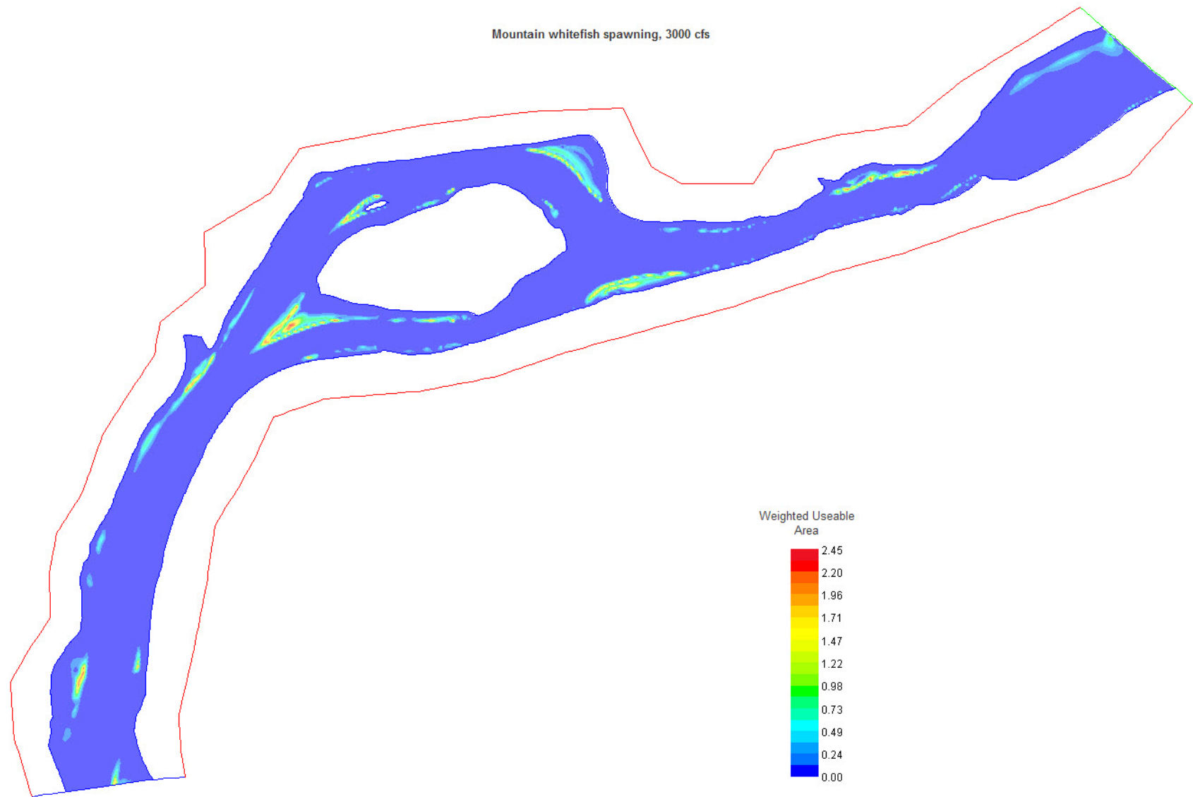
Figure A-92. Mountain whitefish spawning habitat map, Lyons Gulch site, 3000 cfs.
