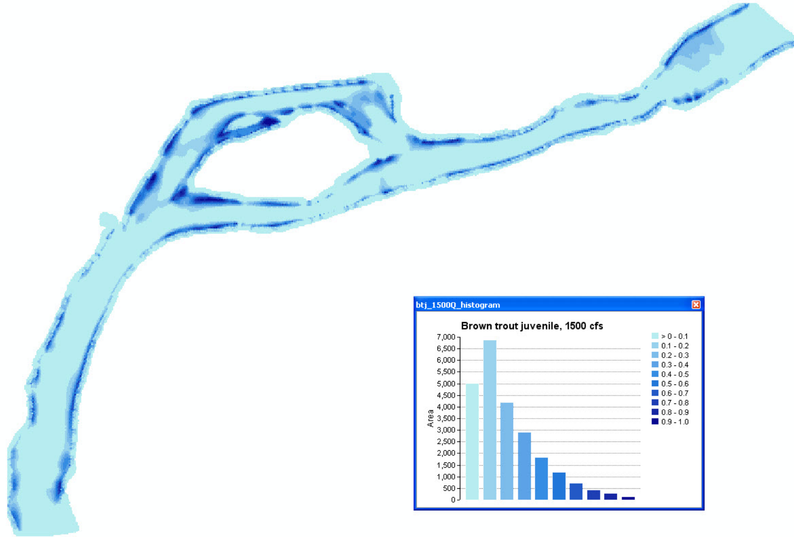
Figure A-67. Juvenile brown trout habitat map, Lyons Gulch site, 1500 cfs.
