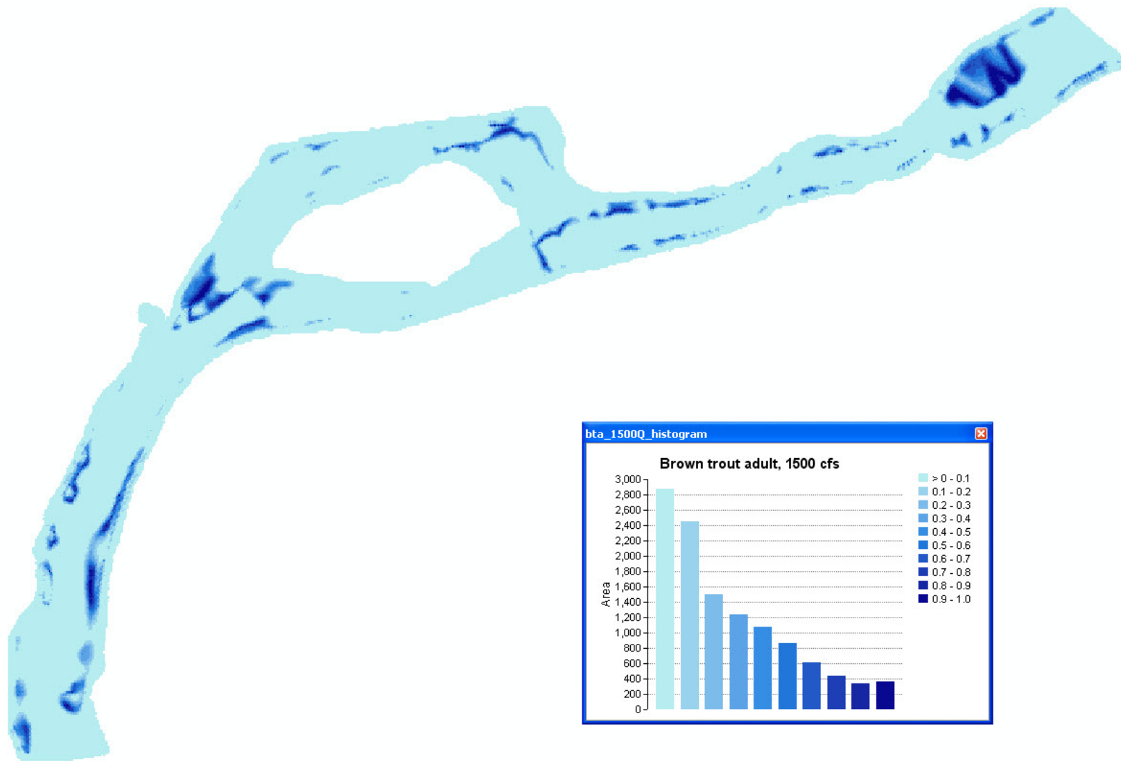
Figure A-64. Adult brown trout habitat map, Lyons Gulch site, 1500 cfs.
