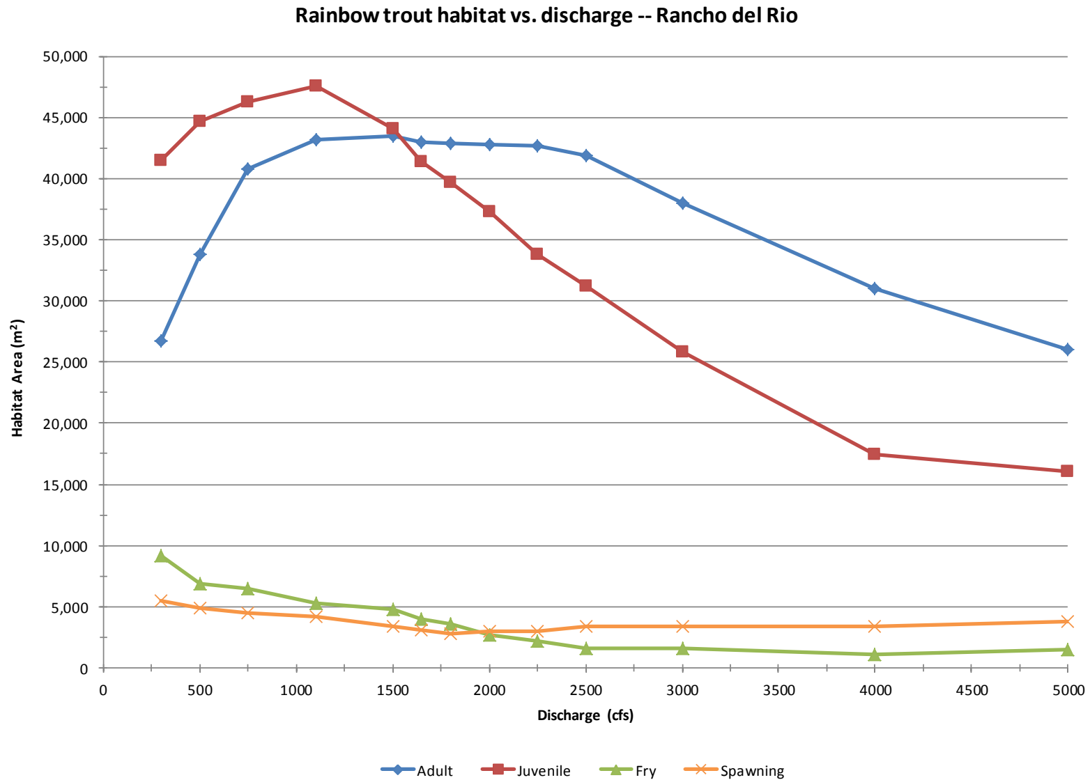
Figure 64. Rainbow trout habitat versus discharge, Rancho del Rio site.
