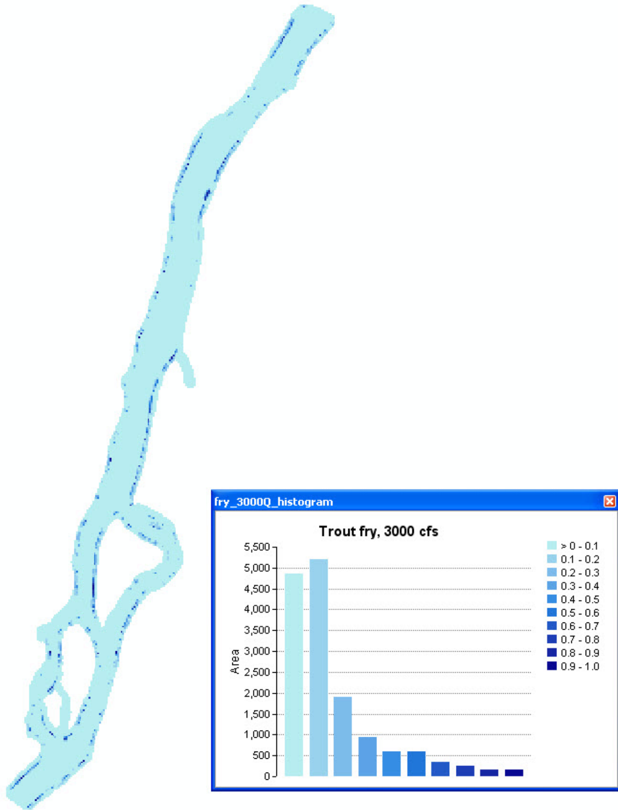
Figure 58. Trout fry habitat map, 3000 cfs, Pumphouse site.
