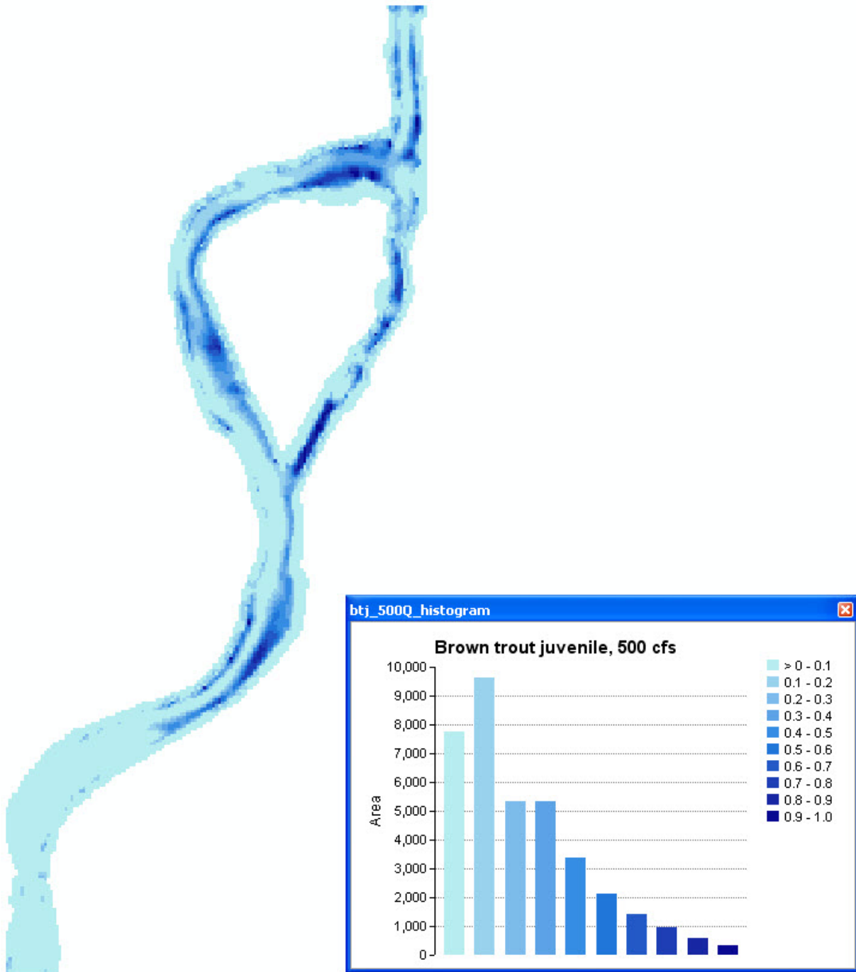
Figure A-33. Juvenile brown trout habitat map, Rancho del Rio site, 500 cfs.
