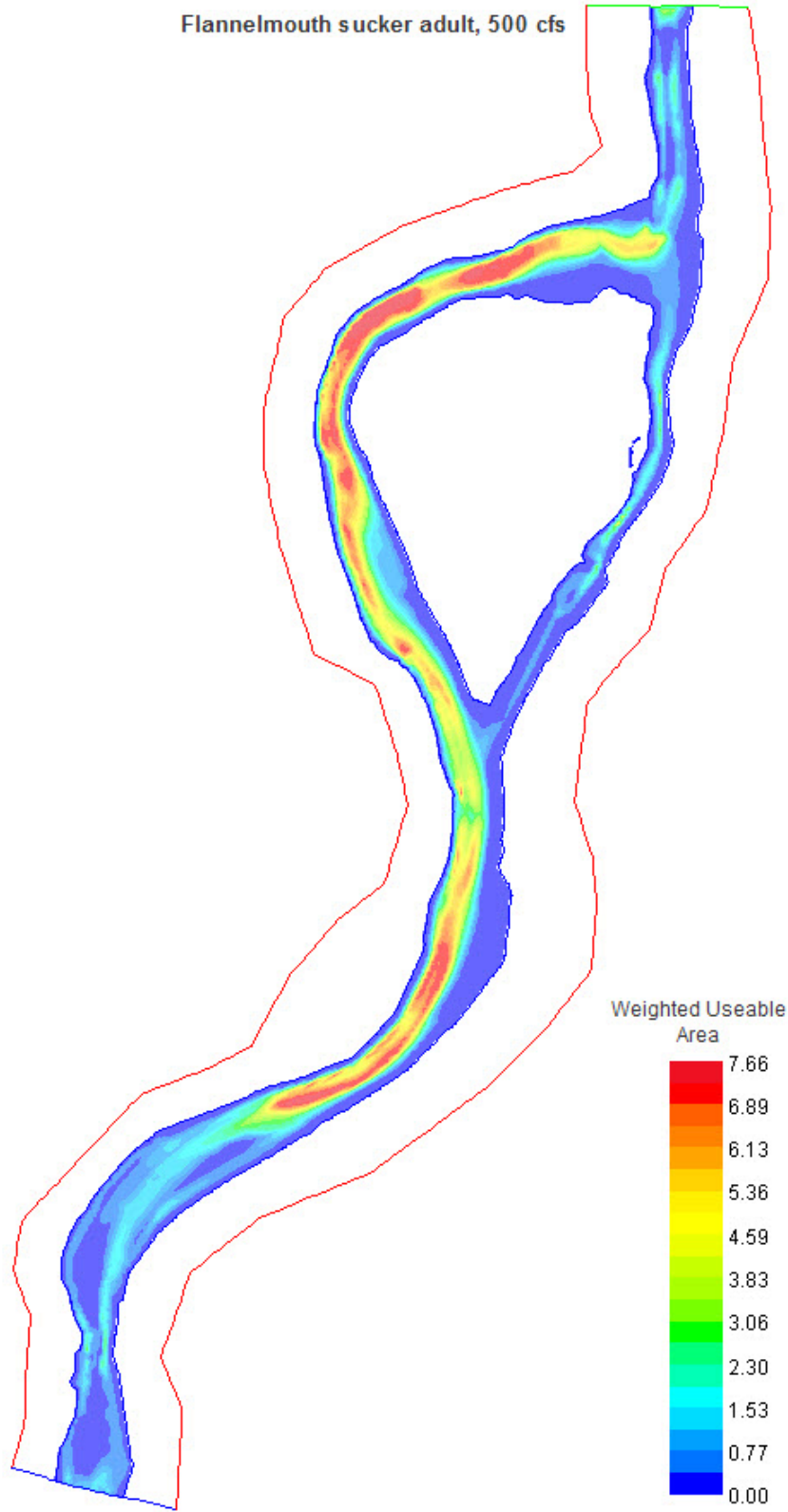
Figure A-60. Adult flannelmouth sucker habitat map, Rancho del Rio site, 500 cfs.
