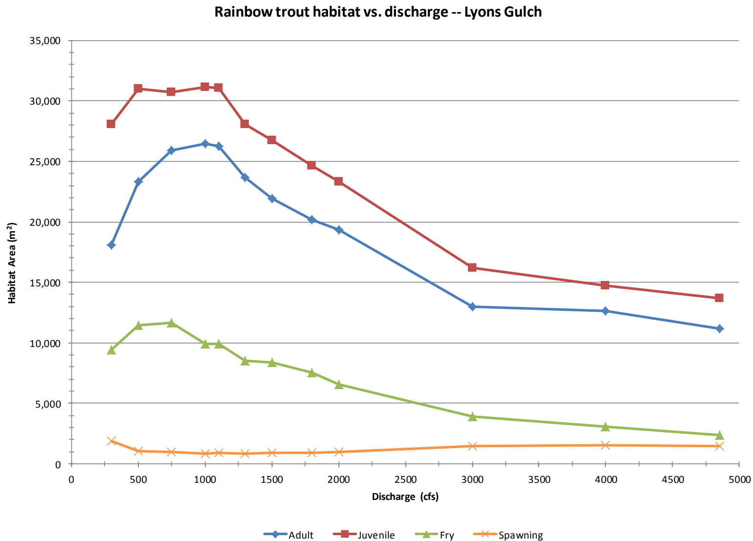
Figure 74. Rainbow trout habitat versus discharge, Lyons Gulch site.
