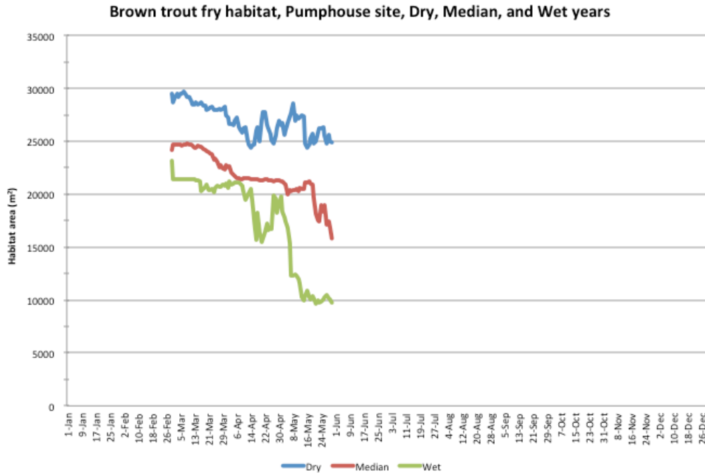
Figure B-3. Brown trout fry habitat time series, dry, median, and wet years, Pumphouse site.
