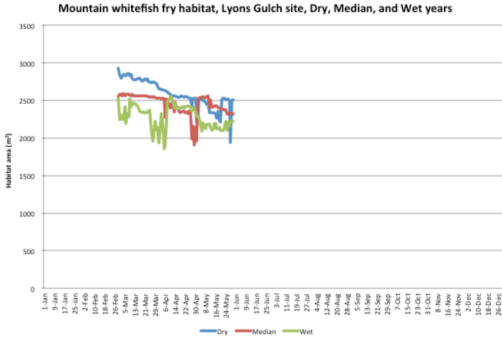
Figure B-36. Mountain whitefish fry habitat time series, dry, median, and wet years, Lyons Gulch site.
