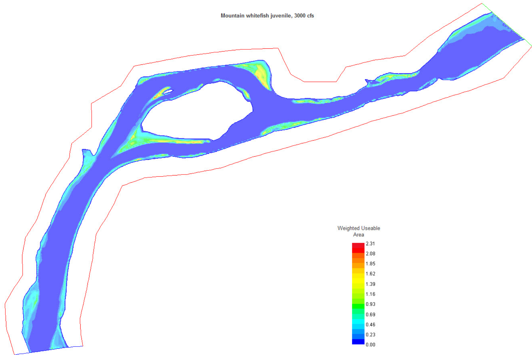
Figure A-86. Juvenile mountain whitefish habitat map, Lyons Gulch site, 3000 cfs.
