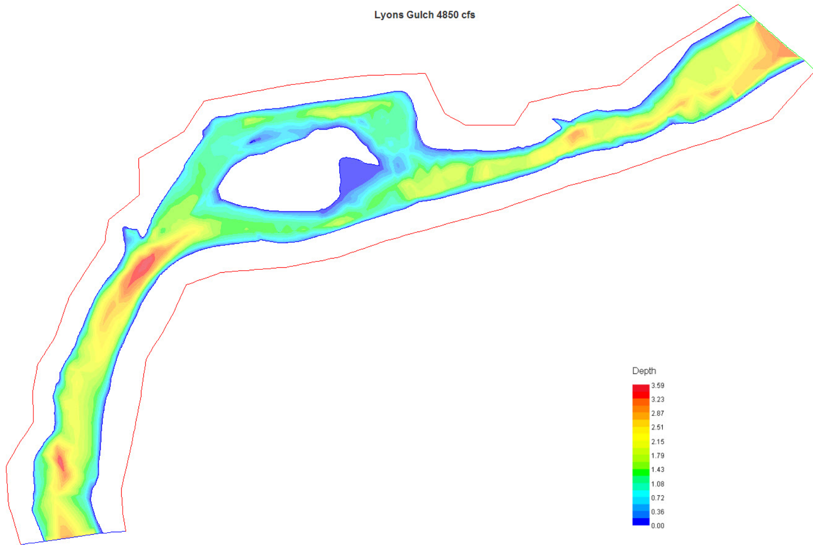
Figure 49. Lyons Gulch simulated water depth (m) at 4850 cfs (high flow). Flow moves from right to left.
