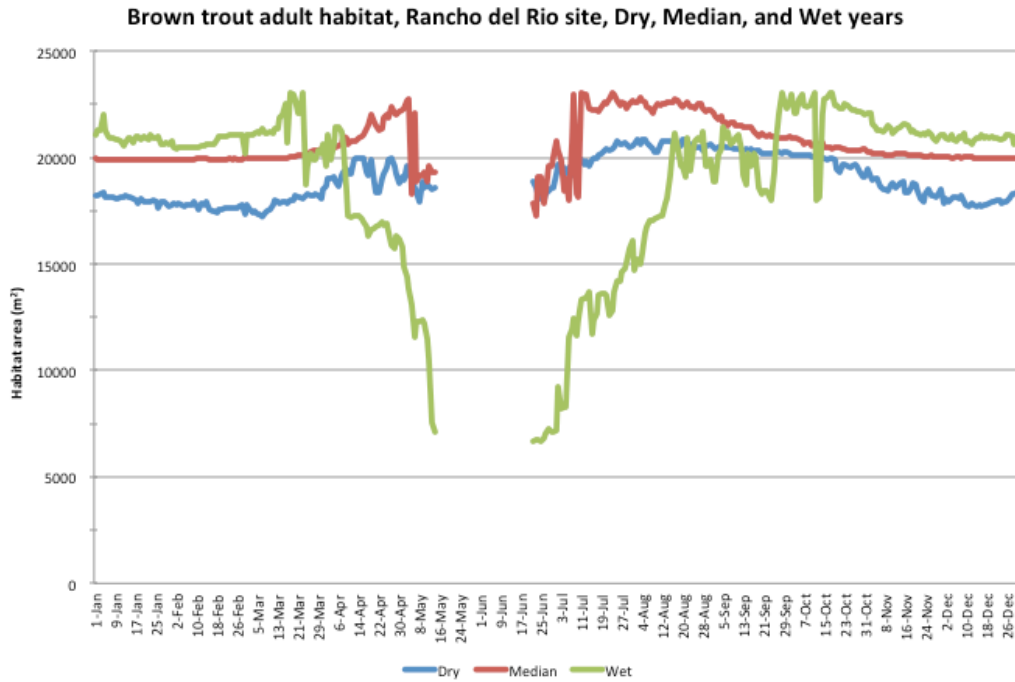
Figure B-13. Adult brown trout habitat time series, dry, median, and wet years, Rancho del Rio site.
