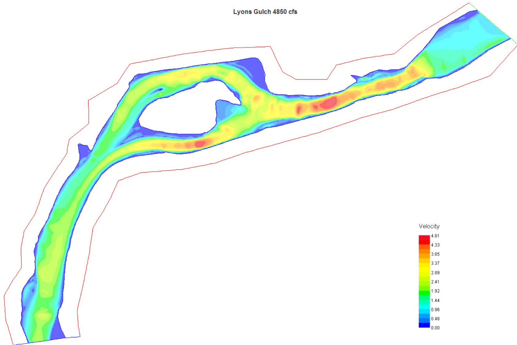
Figure 47. Lyons Gulch simulated water velocity (m/s) at 4850 cfs (high flow). Flow moves from right to left.
