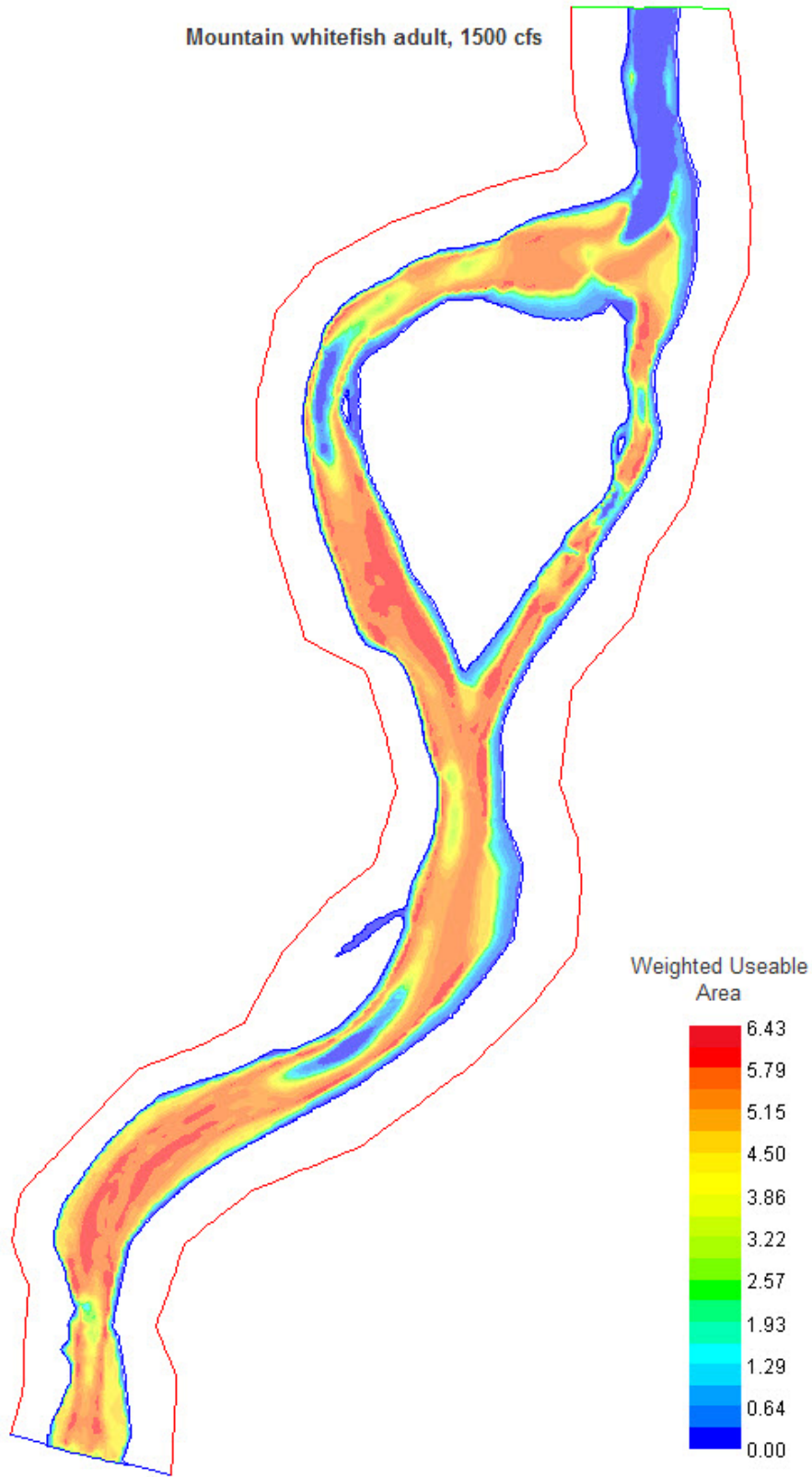
Figure A-49. Adult mountain whitefish habitat map, Rancho del Rio site, 1500 cfs.
