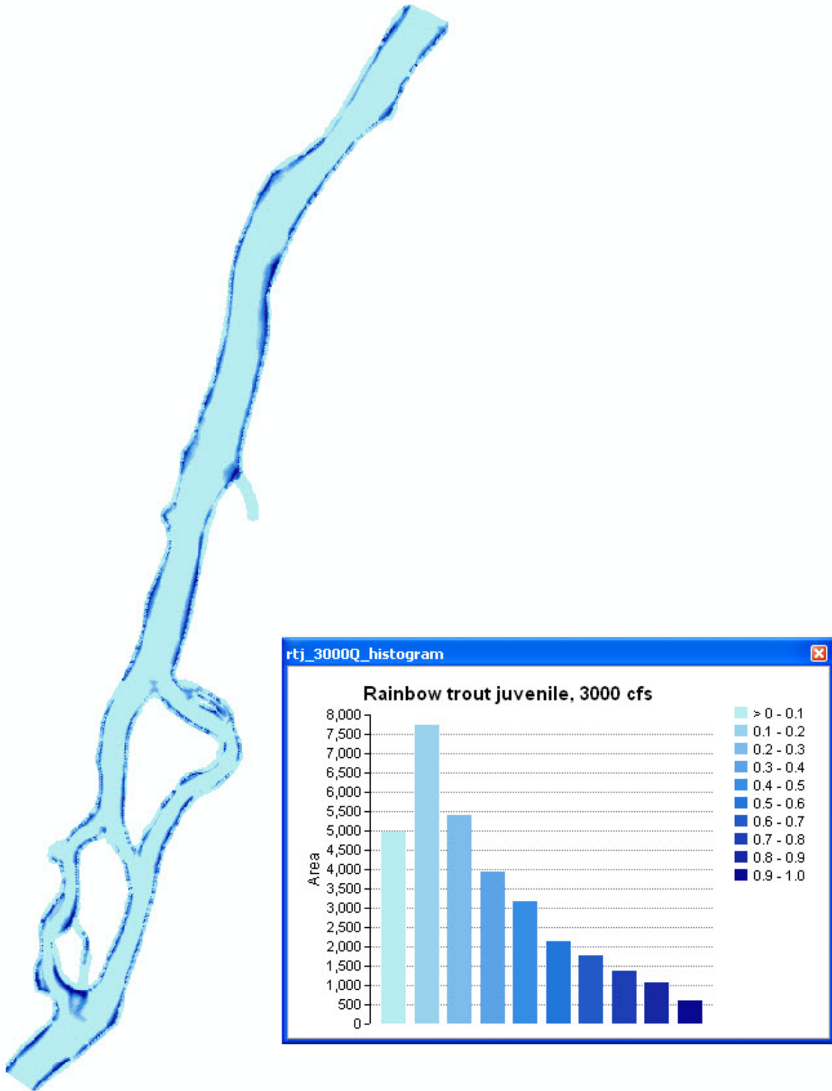
Figure A-12. Juvenile rainbow trout habitat map, Pumhouse site, 3000 cfs.
