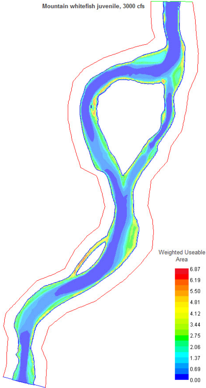
Figure A-53. Juvenile mountain whitefish habitat map, Rancho del Rio site, 3000 cfs.
