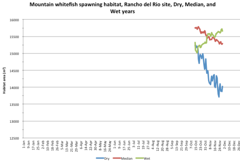
Figure B-24. Mountain whitefish spawning habitat time series, dry, median, and wet years, Rancho del Rio site.
