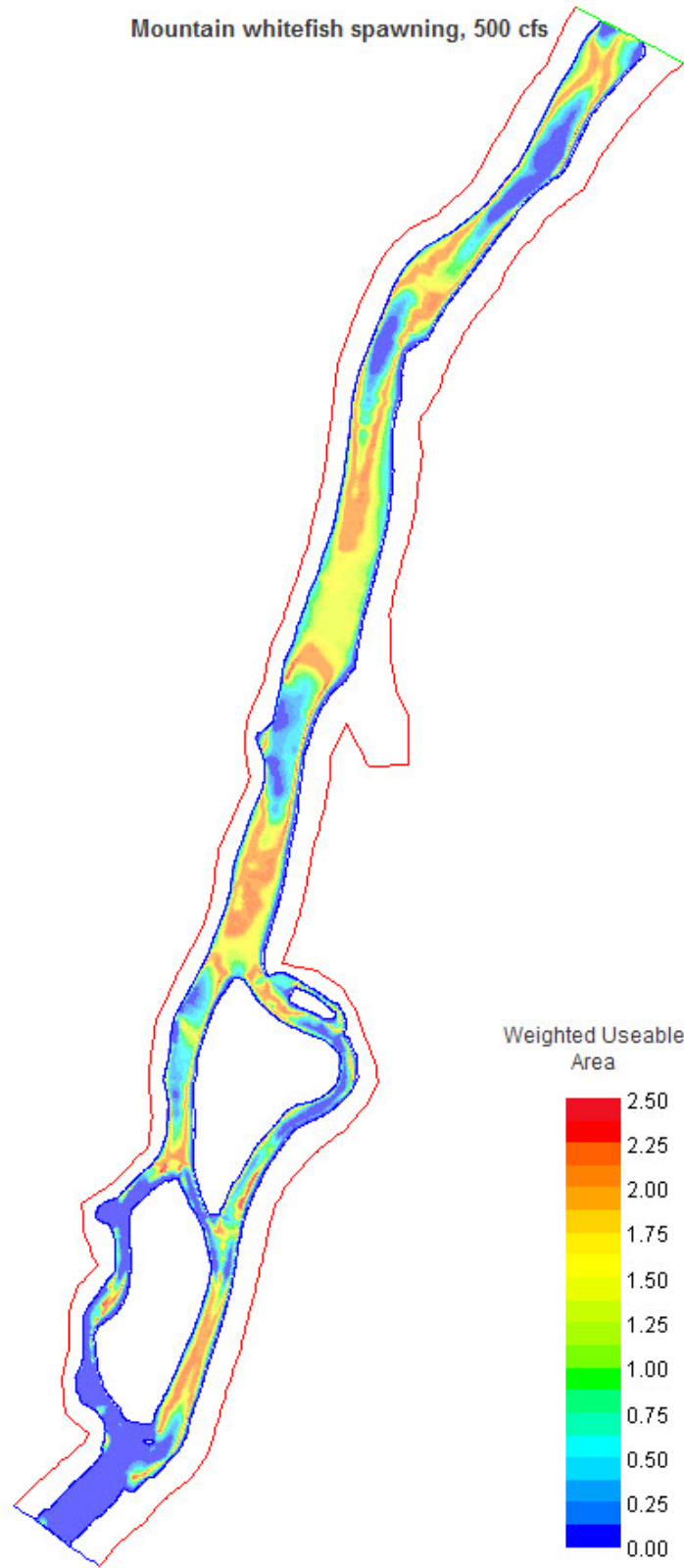
Figure A-27. Mountain whitefish spawning habitat map, Pumphouse site, 500 cfs.
