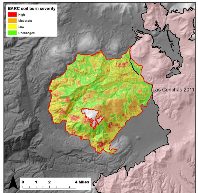
Figure 11. BARC soil burn severity map for the Thompson Ridge Fire.
