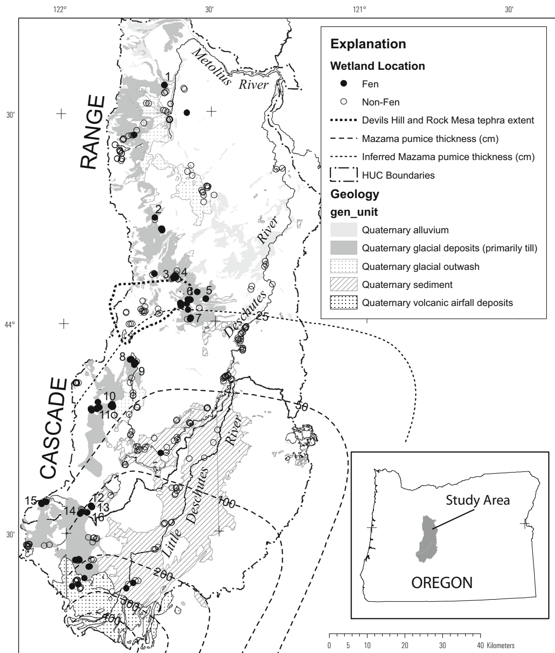
Fig. 1 Field inventoried wetlands, Quaternary surficial sedimentary deposits, and distribution of major tephra in the western half of the upper Deschutes Basin, central Oregon. Line showing the extent of the Devils Hill and Rock Mesa tephra corresponds to the 10 cm thickness
