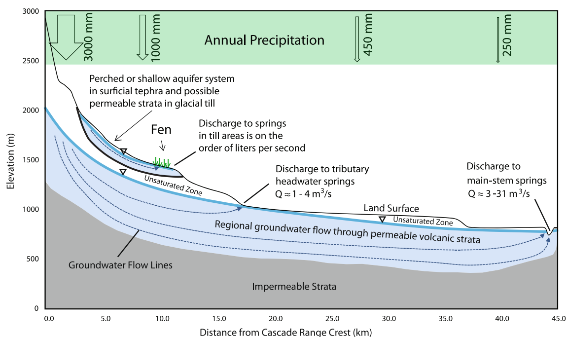
Fig. 5 Diagram showing conceptual cross section from the Cascade Range crest east to the main stem of the Deschutes River. The water table is marked by inverted triangles. An unsaturated zone is shown
