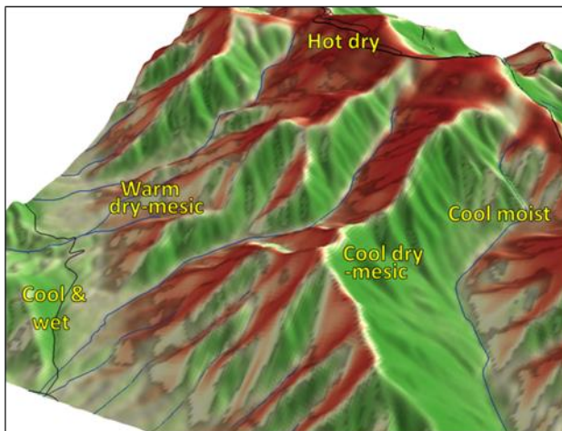
Figure 8c: A draped 30m grid of solar radiation values. The green-to-red color gradient indicates low solar inputs to high. Heat-loading is highest on south-to-west facing steep upper slopes and ridges, while north-facing slopes and shaded areas are protected from sun effects. Environmental conditions, ecological processes, and natural systems can vary dramatically with the variation in landscape structure show in this and the previous figure.
