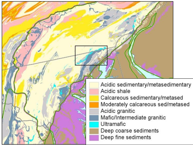
Figure 13a: The Baltimore Mafic Complex. Shaded in cyan, this as a large occurrence of ultramafic bedrock in the southern part of the Lower New England/Northern Piedmont Ecoregion, on the eastern part of the Maryland-Pennsylvania.
