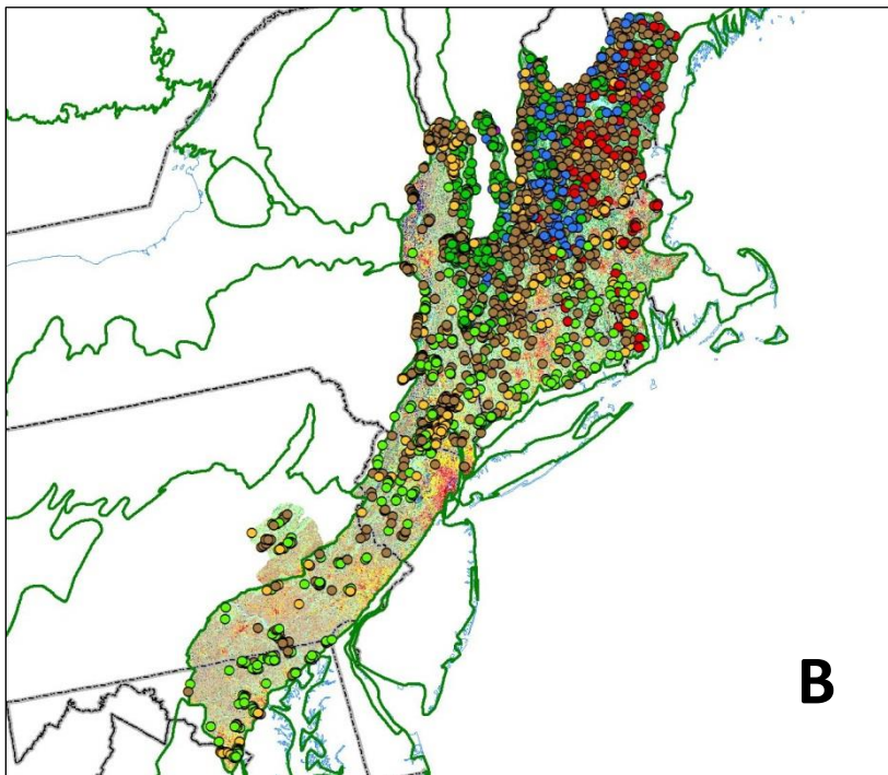
Figure 4a & b: Known sample points for the Lower New England/Northern Piedmont Ecoregion (LNE). In Fig. 4a, FIA plots screened for “naturalness” show an uneven distribution, reflecting patterns of land use across the largely humanized landscapes of this region. The pattern is denser, but the unevenness persists, when all known sample points from all sources are plotted (Fig. 4b).
