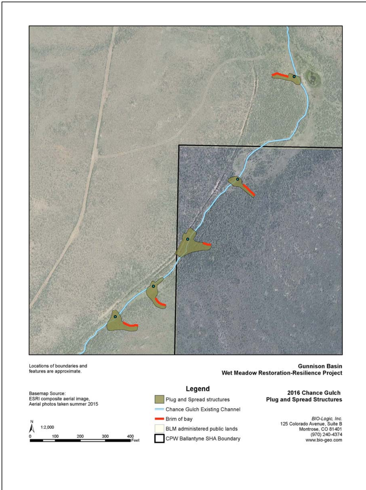
Map 8. Plug and Spread Structures built in late 2016 in the lower reach of Chance Gulch (prepared by Shawn Conner, BIO-Logic, Inc.).
