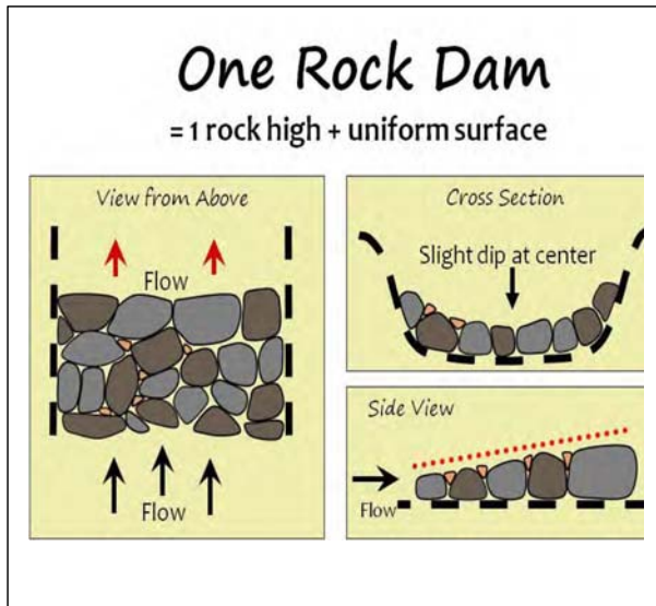
Figure 2. Selected restoration structures used in this project designed by Bill Zeedyk. Sources: Zeedyk (2014), Zeedyk (2015) and Sponholtz and Anderson (2010).
