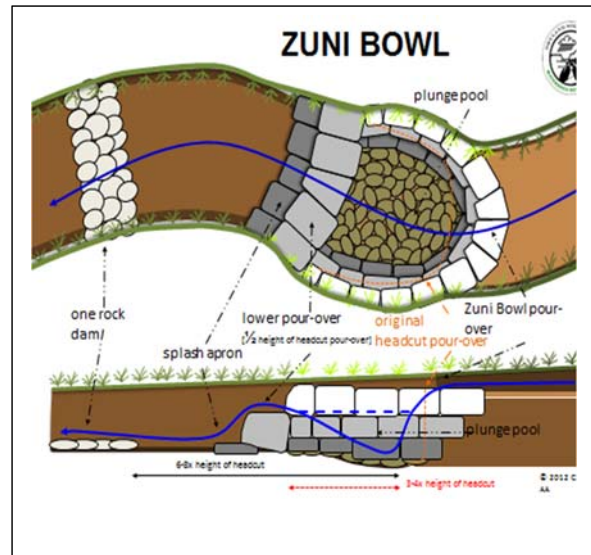
Figure 2. Selected restoration structures used in this project designed by Bill Zeedyk. Sources: Zeedyk (2014), Zeedyk (2015) and Sponholtz and Anderson (2010).
