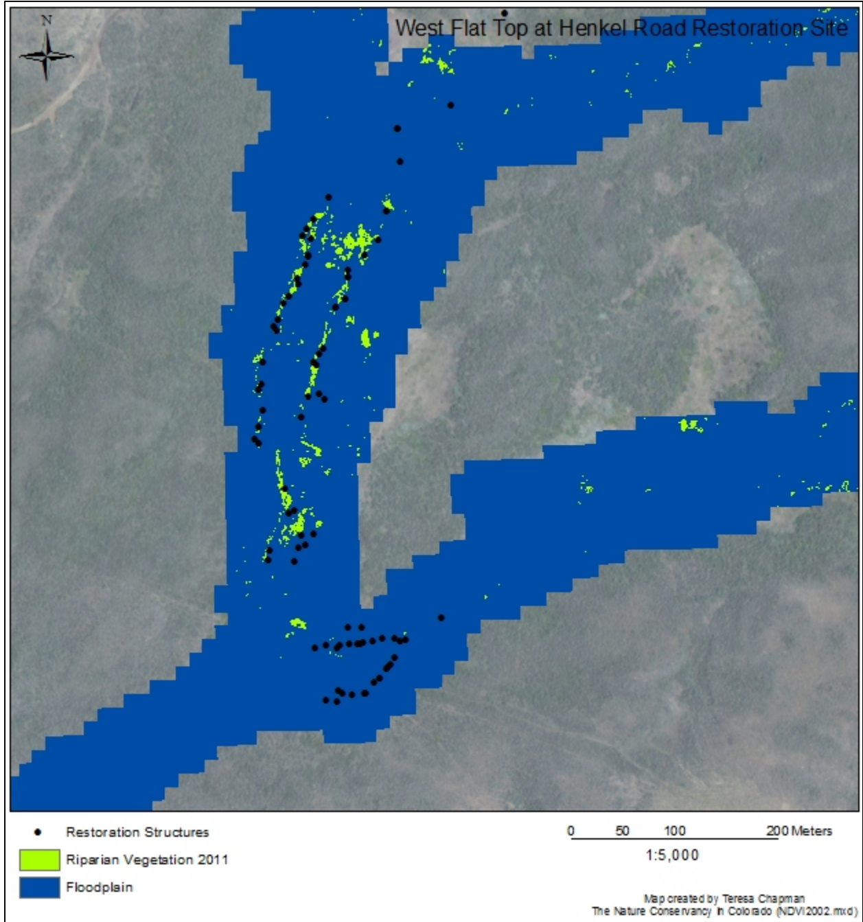
Figure 10. Extent of riparian vegetation in 2011 prior to restoration overlaid with topography based modeled floodplain at West Flat Top at Henkel Road restoration site. The ratio of 2011 riparian vegetation to the area of the floodplain creates the Riparian Condition Index and estimates the potential for expansion of the wetland.
