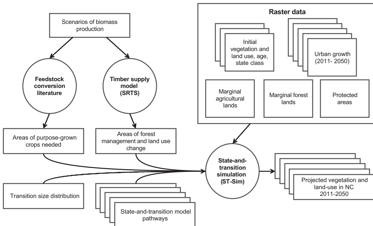
Fig. 1 Conceptual overview of model flow. Narrative scenarios about biomass production were translated into annual areas of land-use change and management via information in the feedstock conversion literature and the Sub-Regional Timber Supply model. Raster data sets were used to initialize the landscape, constrain purpose-grown crops to marginal agricultural or forest lands, direct urban growth, and exclude protected areas from biomass harvest. Raster data and areas of land-use change and management, along with transition size distributions, state-and-transition model pathways, were input into ST-Sim to produce maps of landscape change.
