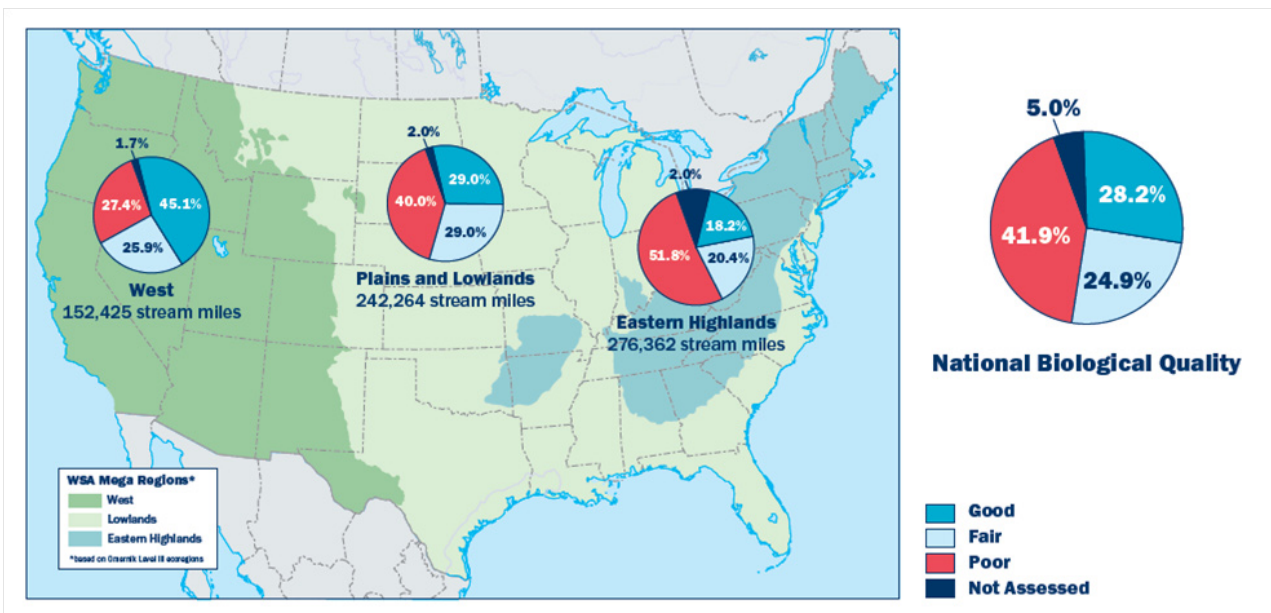
Figure 3-31 Biological quality results from EPA's Wadeable Streams Assessment (U.S. Environmental Protection Agency, 2008c).
