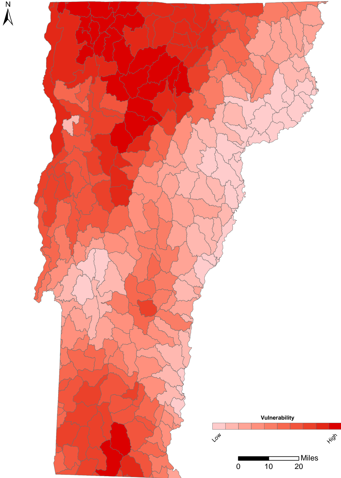
Figure 4-12 Relative watershed vulnerability scores for Vermont.
