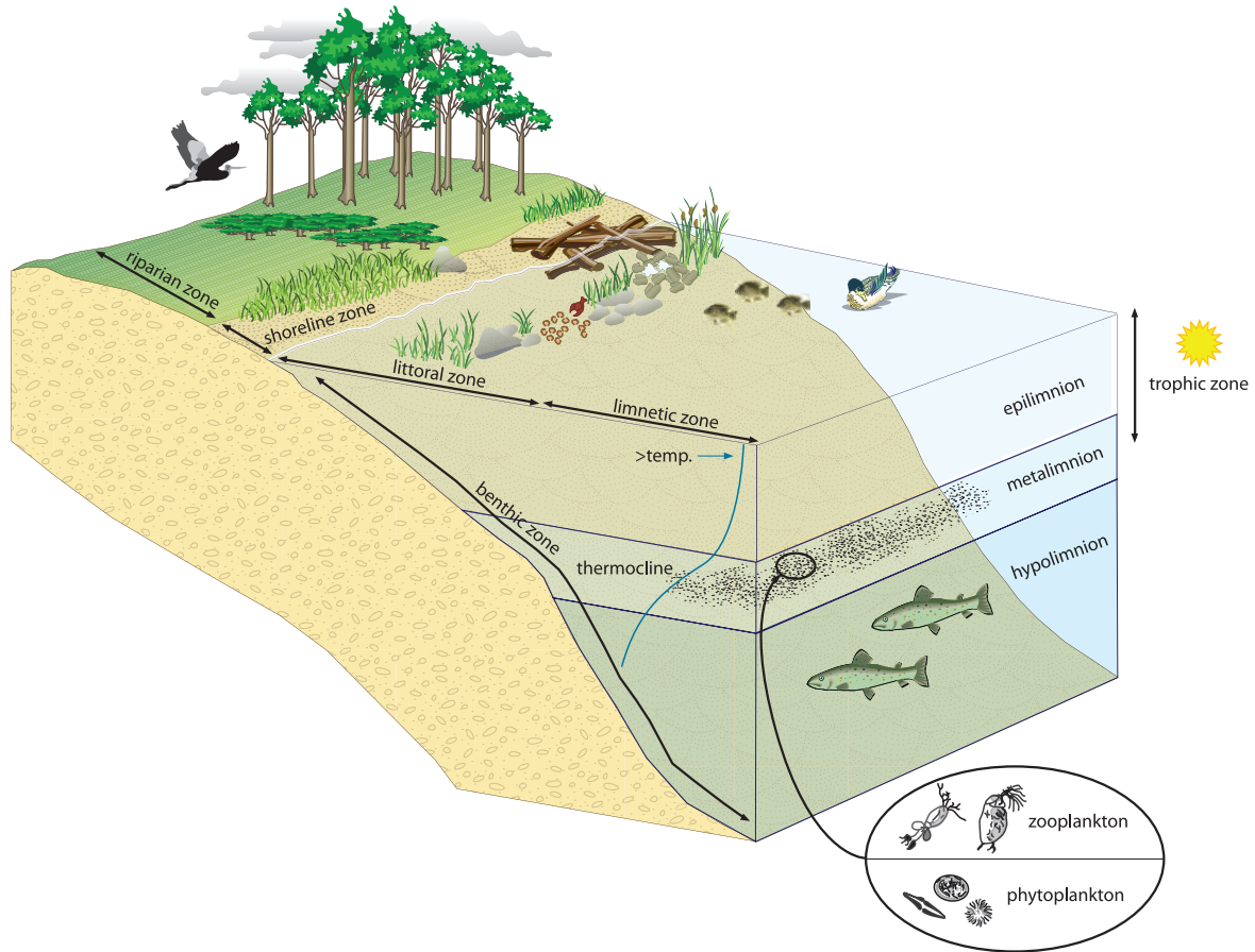
Figure 2-14 Schematic of a lakeshore and the three habitat zones of a typical lake (U.S. Environmental Protection Agency, 2009a).
