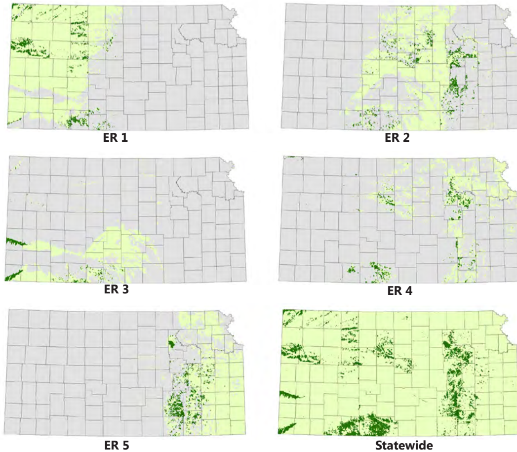
Figure 4-27 Location of least disturbed watersheds within individual quantitative ecoregions (ER) (k = 5) (Angelo, Knight, Olson, & Stiles, 2010). Rankings are based on the disturbance index derived via principal components analysis. Highlighted watersheds rank in the lowest (best) 10th percentile within their respective ecoregions. The statewide (10th percentile) map is shown for comparison.
